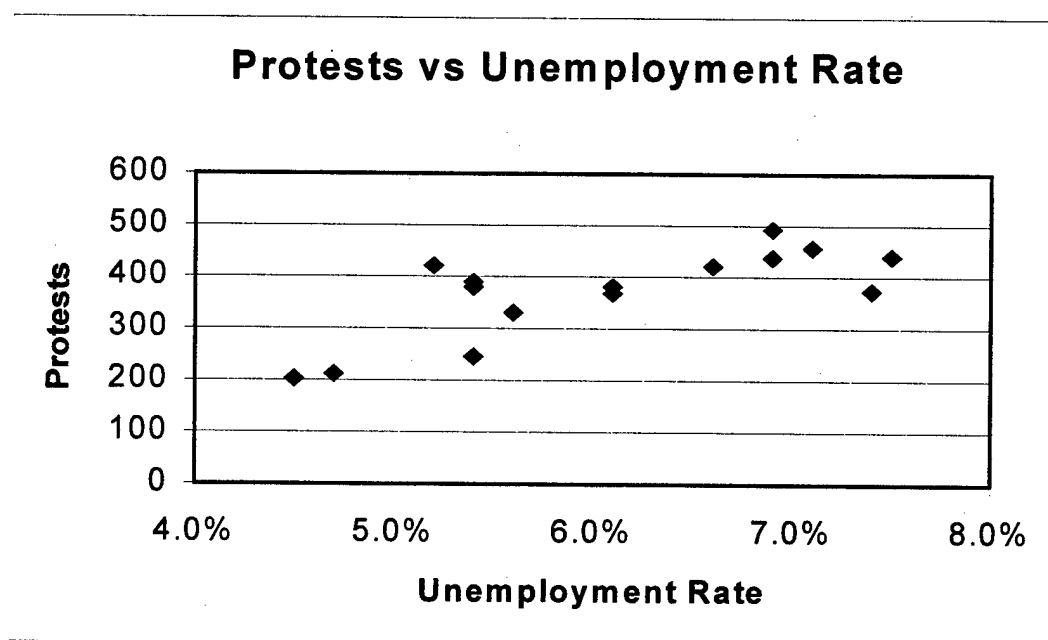
Figure 7: AF GAO-Protests Processed vs. Unemployment Rate Scattergram
