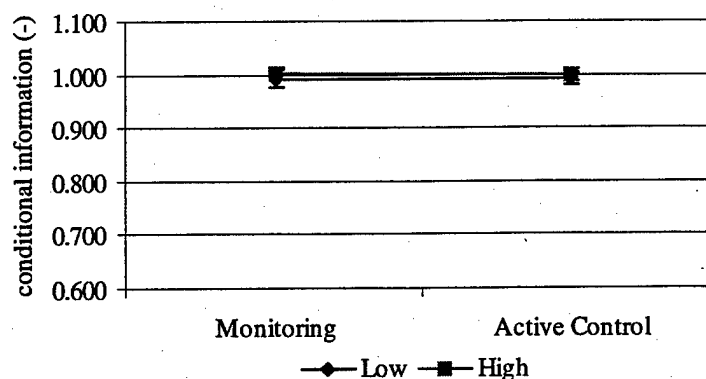
Figure 17. Range-based conditional information index by load and involvement.
