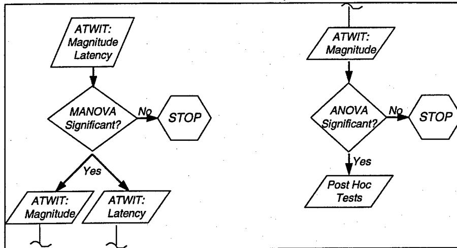
Figure 2. Statistical analysis.
