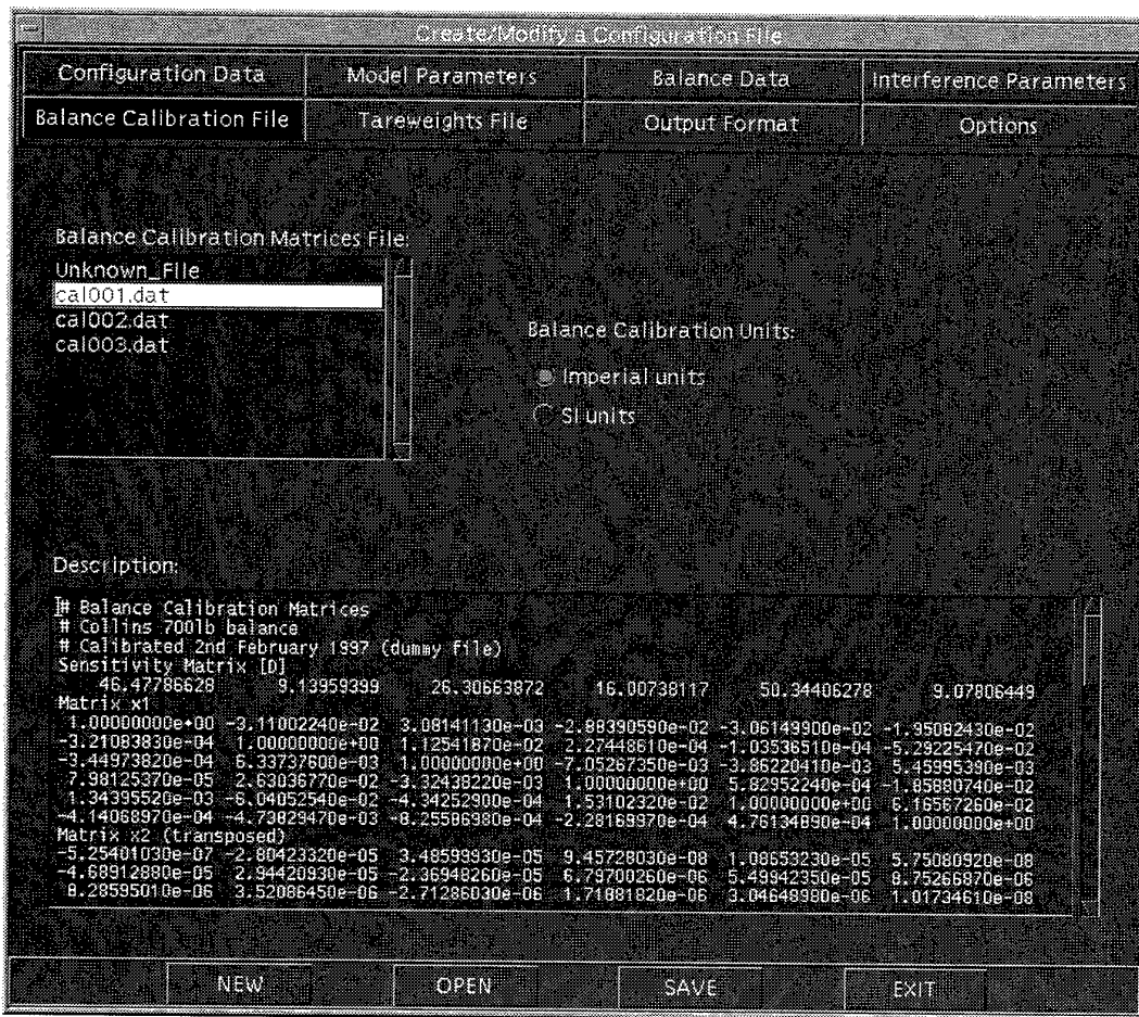
Figure 8. Balance Calibration File page for the Configuration File Editor
