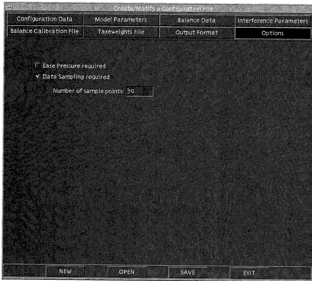
Figure 11. Options page for the Configuration File Editor
