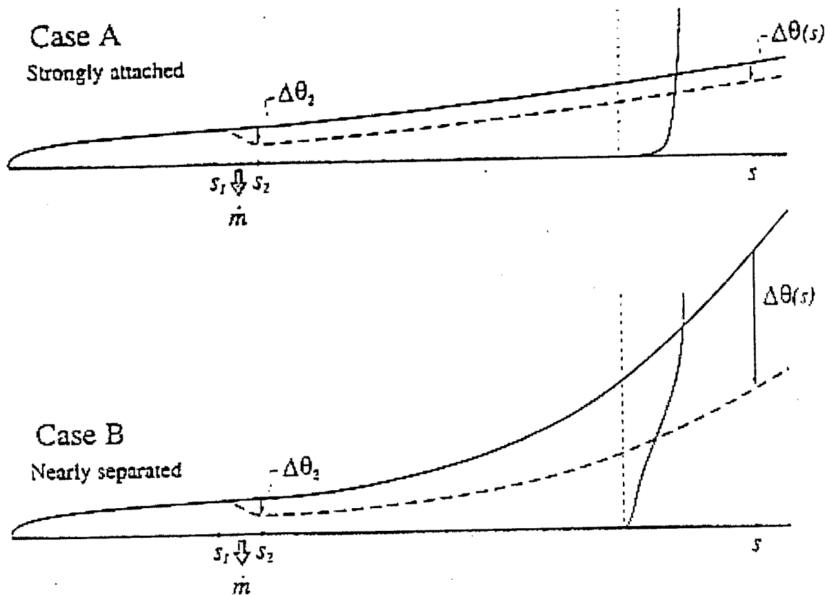
Figure 1-2: Effect of suction on boundary layer growth
