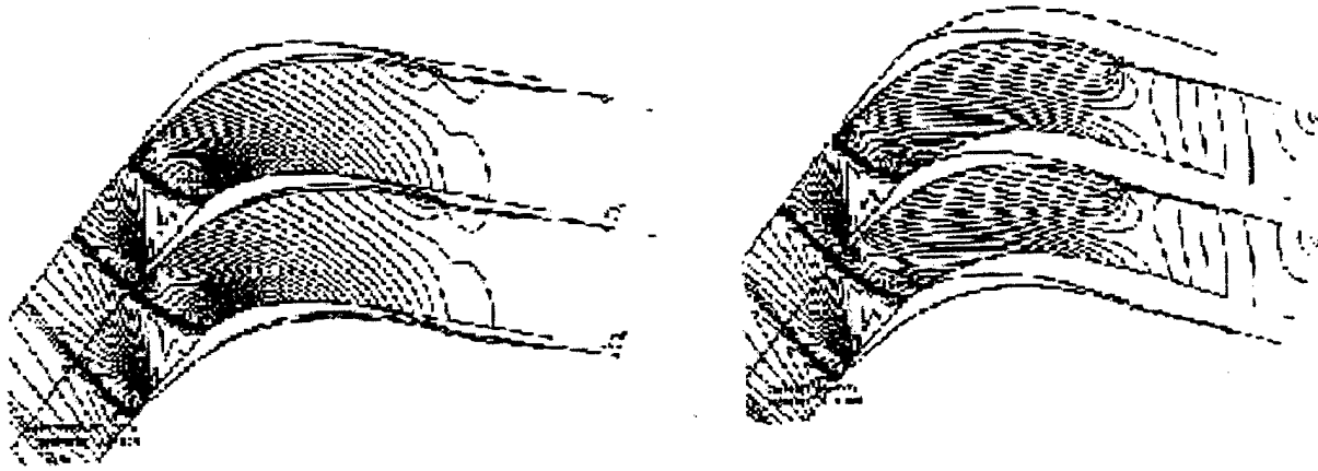
Figure 1-1: Comparison of Same Airfoil shown with and without Suction
