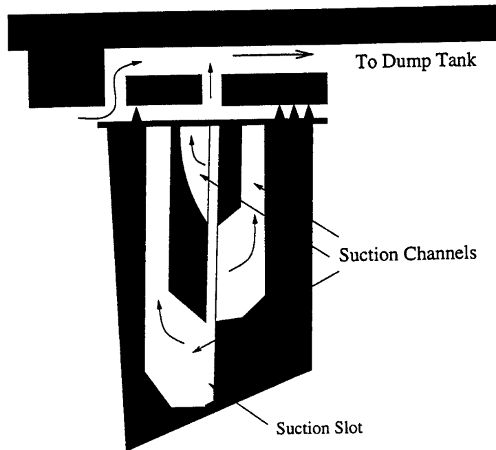
Figure 2-2: Schematic of Suction Flow Transport System
