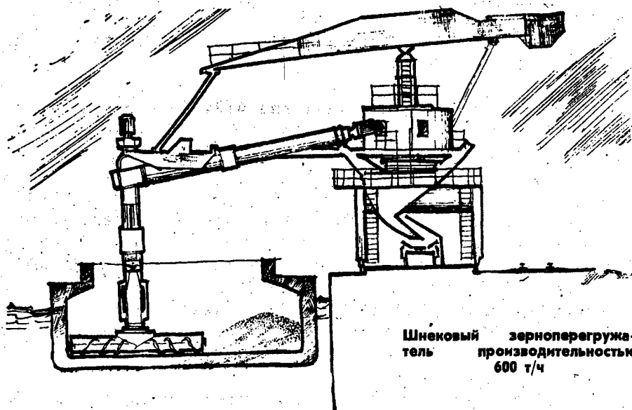
An auger-type grain transshipper having a productivity of 600 tons per hour.
