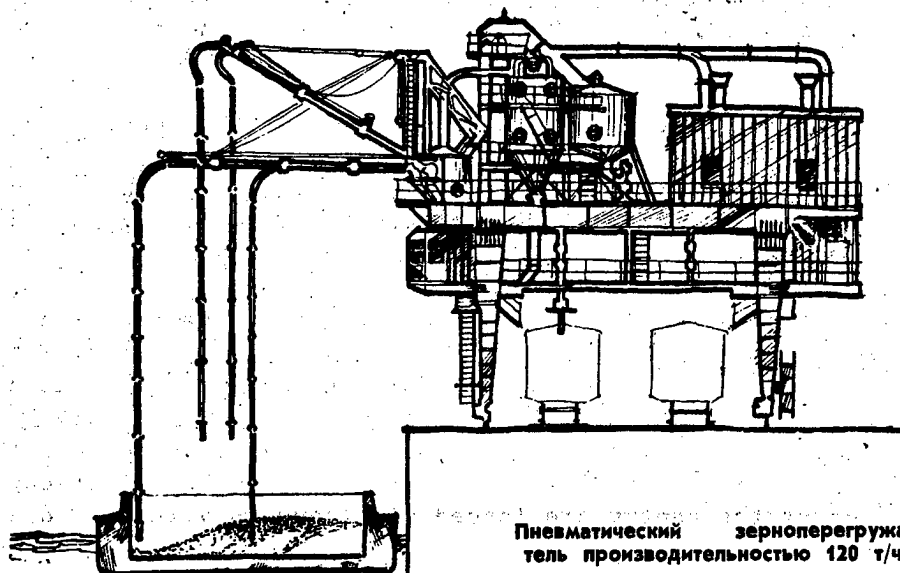
A pneumatic grain transhipper having a productivity of 120 tons per hour.
