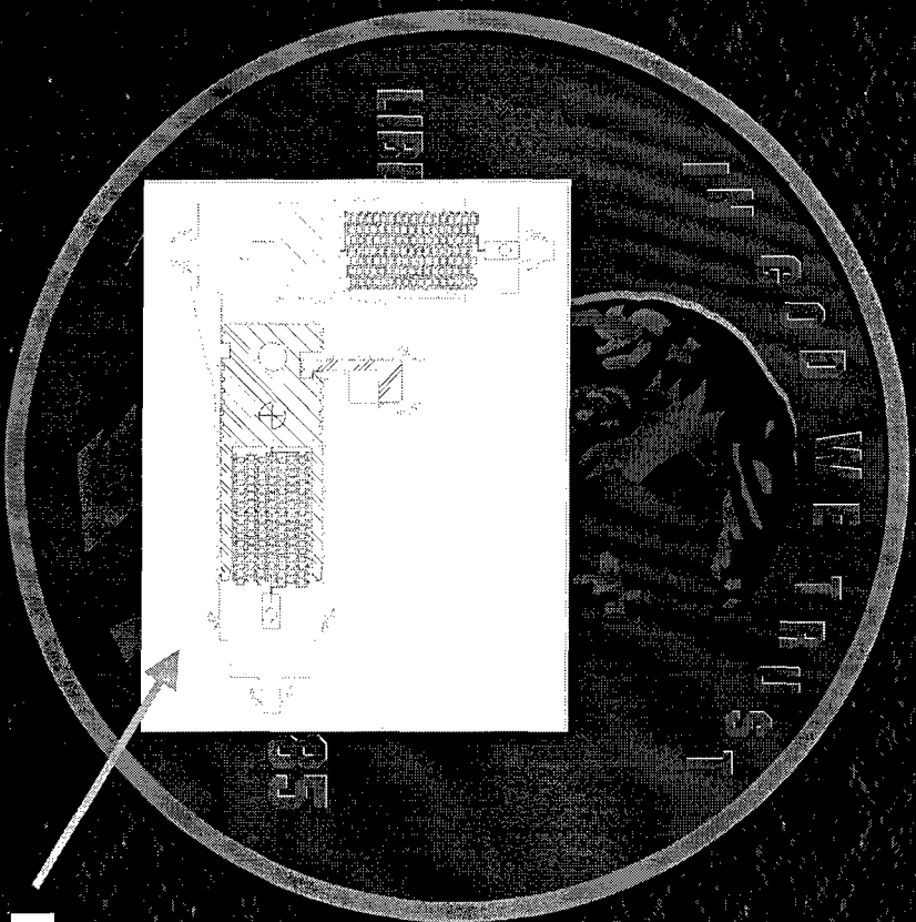
MEMS Mechanical S&A Chip
