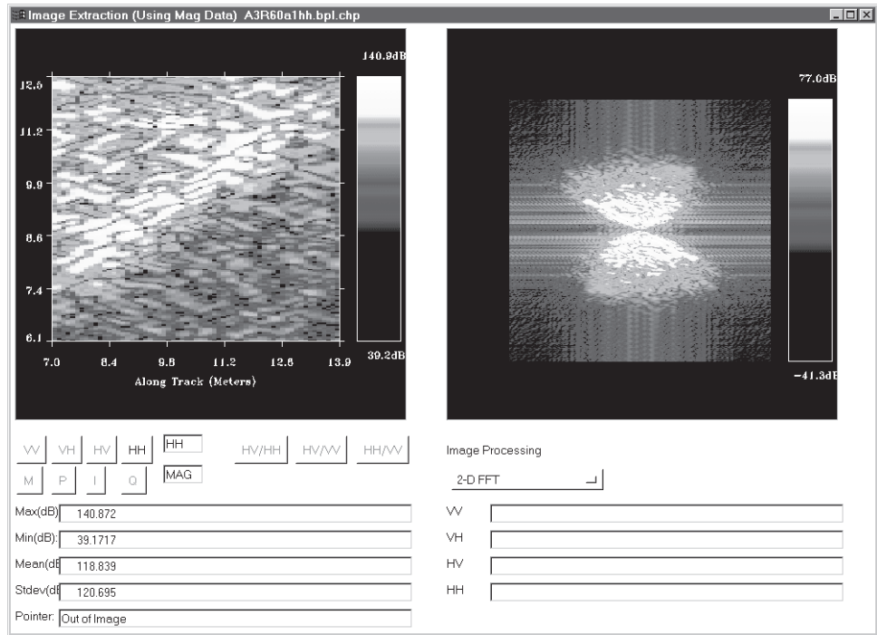
Figure 39. Image of vehicle and its 2-D FFT visualization.
