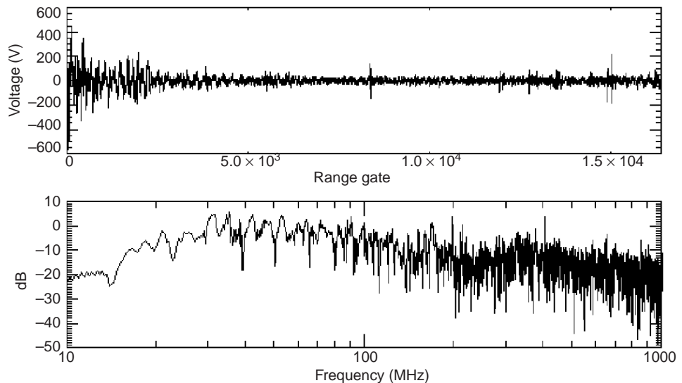
Figure 12. Radar data after RFI is applied. Note that RFI level is reduced compared to that of figure 11.
