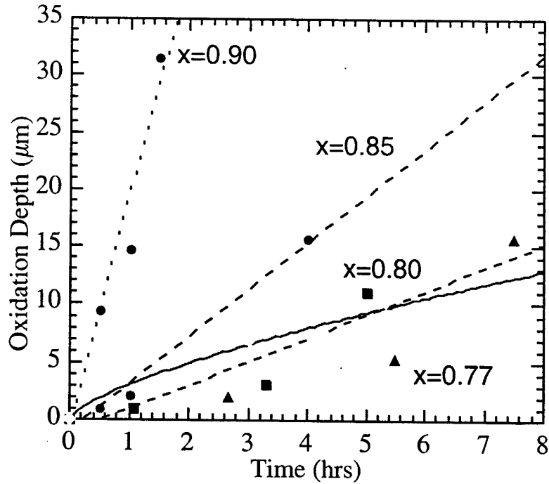
Figure 4.7: Temporal dependence of the lateral oxidation depth of AlGaAs ( x > 0.77 ) at 475°C. The solid line shows the corresponding dependence for \text{In}_{0.48}\text{Al}_{0.52}\text{As} .
