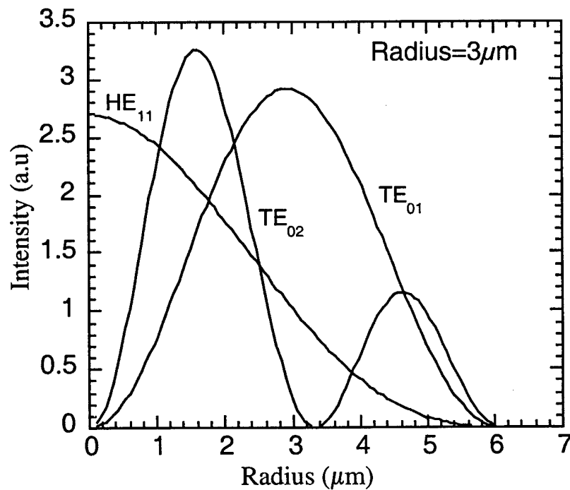
Figure 4.10: Transverse mode profile for a VCSEL (radius=6μm) for (a) HE 11 , (b) TE 01 , and (c) TE 02
