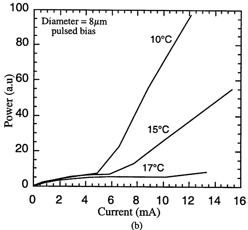
Figure 5.2: (a) Threshold current vs device diameter at 15^\circ\text{C} and, (b) temperature dependence of the light-current characteristic for an 8\mu\text{m} device, under pulsed bias conditions.
