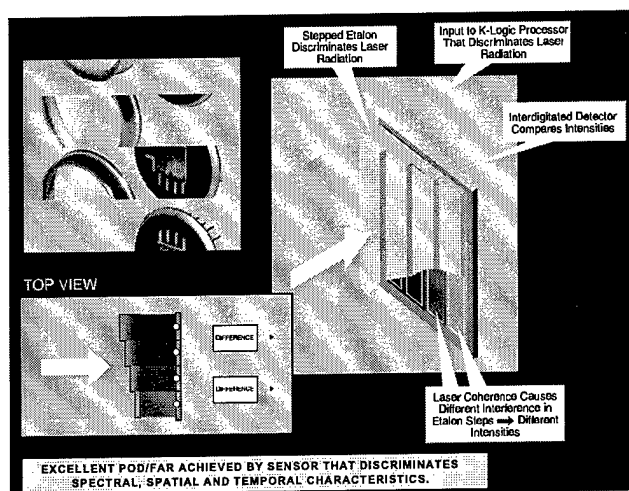
Figure 2. Raytheon Etalon Architecture
