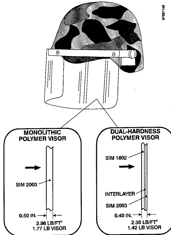
Figure 7. (U) High-performance helmet visor designs.
