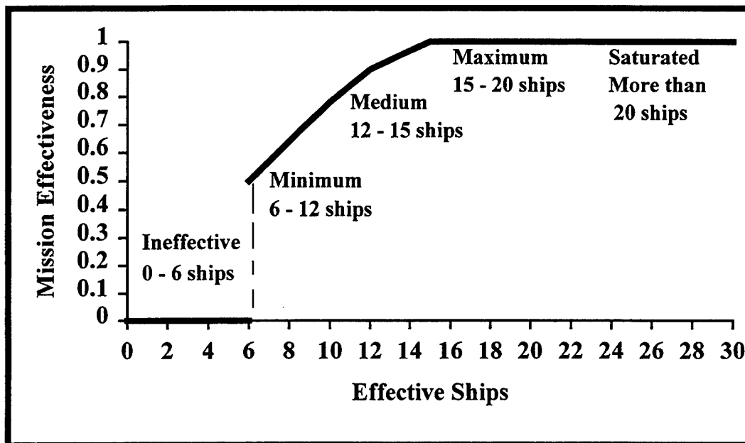
Figure 7. Mission Effectiveness as A Function of Effective Ships Assigned. This graph demonstrates the S curve relationship between mission effectiveness and effective ships assigned for Theater Ballistic Missile Defense in the DEFEND phase. At least 6 effective ships are required to achieve minimum requirements. Mission effectiveness increases rapidly as additional ships are added and reaches .9 once 12 effective ships are assigned. Additional ships only marginally improve effectiveness. No benefit is attained by adding ships at the SATURATED level.
