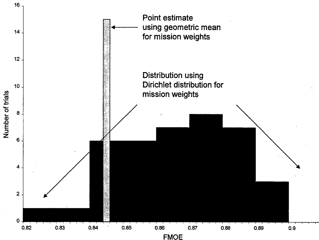
Figure 12. A distribution of FMOE expresses the uncertainty associated with measuring fleet effectiveness. A point estimate using the geometric mean for mission weights does not display this variability.
