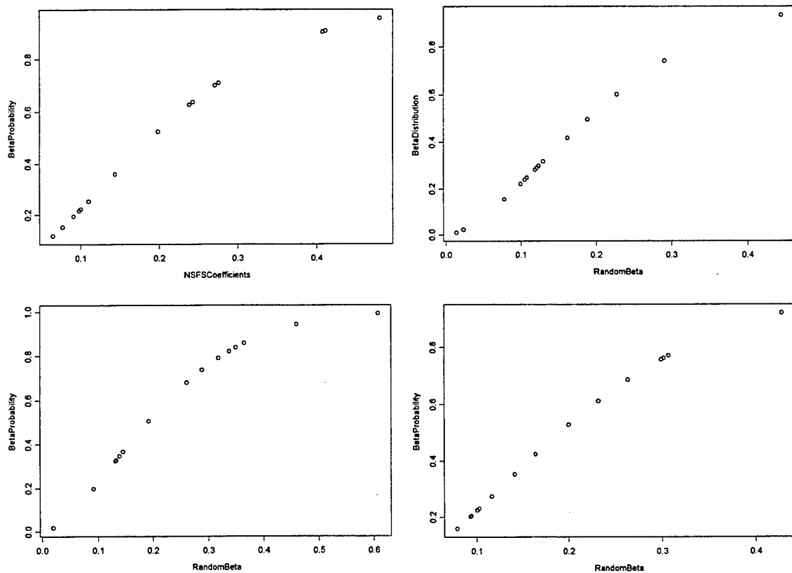
Figure 10. Beta Probability Plots. The graph in the upper left corner gives Beta probability plots for the NSFS weights in phase BUILDUP derived from the decision-makers who completed the mission importance survey (Appendix A). For comparison, three additional Beta probability plots are included, each of 15 randomly generated observations from a Beta (1.76, 6.47). Because these plots appear similar, the Beta distribution is a sensible choice to approximate the marginal distribution of AHP weights.
