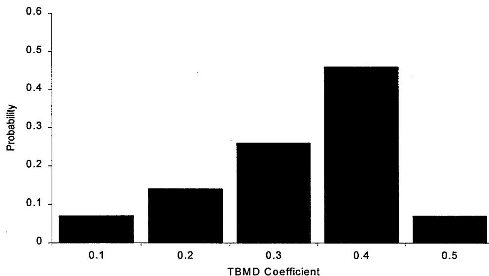
Figure 8. The Histogram of Theater Ballistic Missile Defense Weights in the Phase COUNTER-OFFENSIVE.
