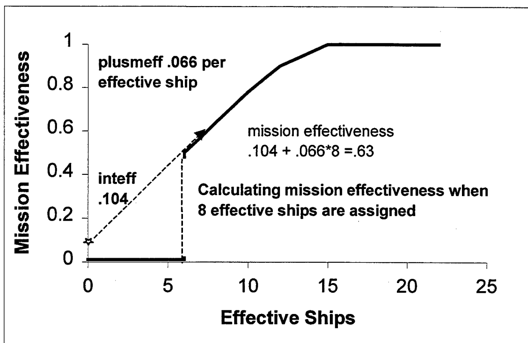
Figure 11. Computation of Mission Effectiveness. The piecewise linear function for mission effectiveness (see Figure 7) is calculated using binary and continuous variables. This figure illustrates how mission effectiveness is calculated if 8 effective ships are assigned TBMD in the Eastern Sea of Japan for phase BUILDUP.
