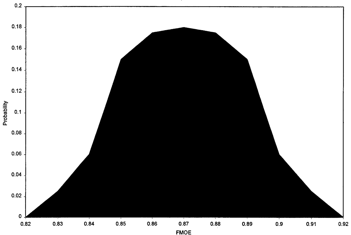
Figure 9. The Notional Distribution of FMOE for a Fleet of 17 CG's, 37 DDG's, and 12 DD's
