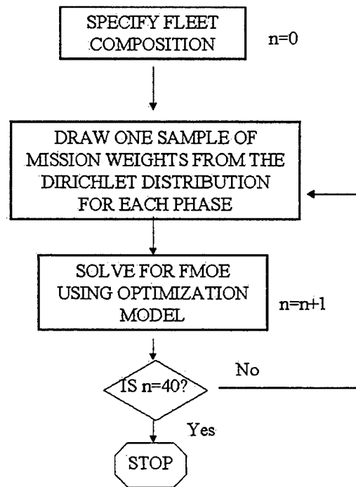
Figure 13. This diagram illustrates the process of computing Fleet Measure of Effectiveness (FMOE) 40 times for a fixed fleet of ships.
