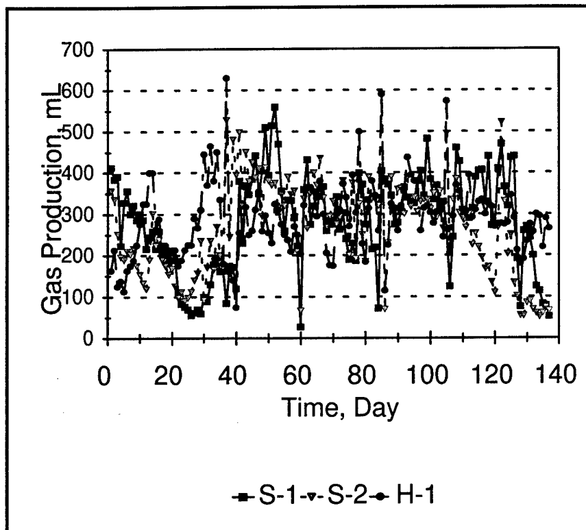
Figure 21. Gas production in single-stage staged-feed system.
