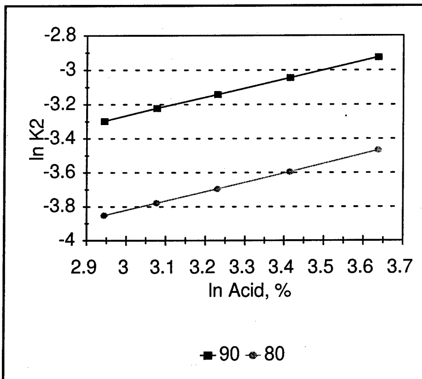
Figure 32. Effect of acid concentration on glucose degradation.
