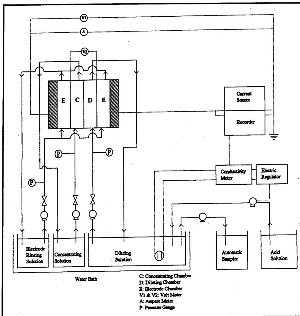
Figure 38. Experimental apparatus for electro dialysis (Urano et al. 1984).
