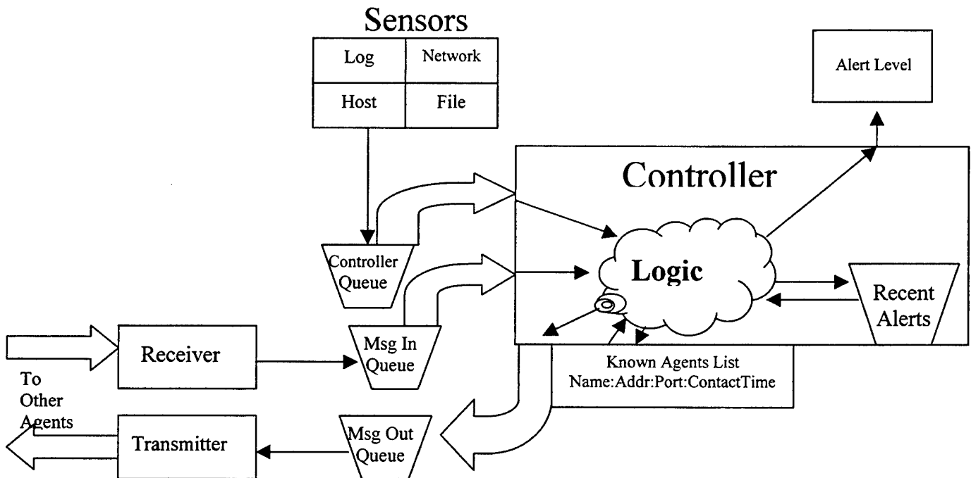
Figure 1: IDAgent Block Diagram
