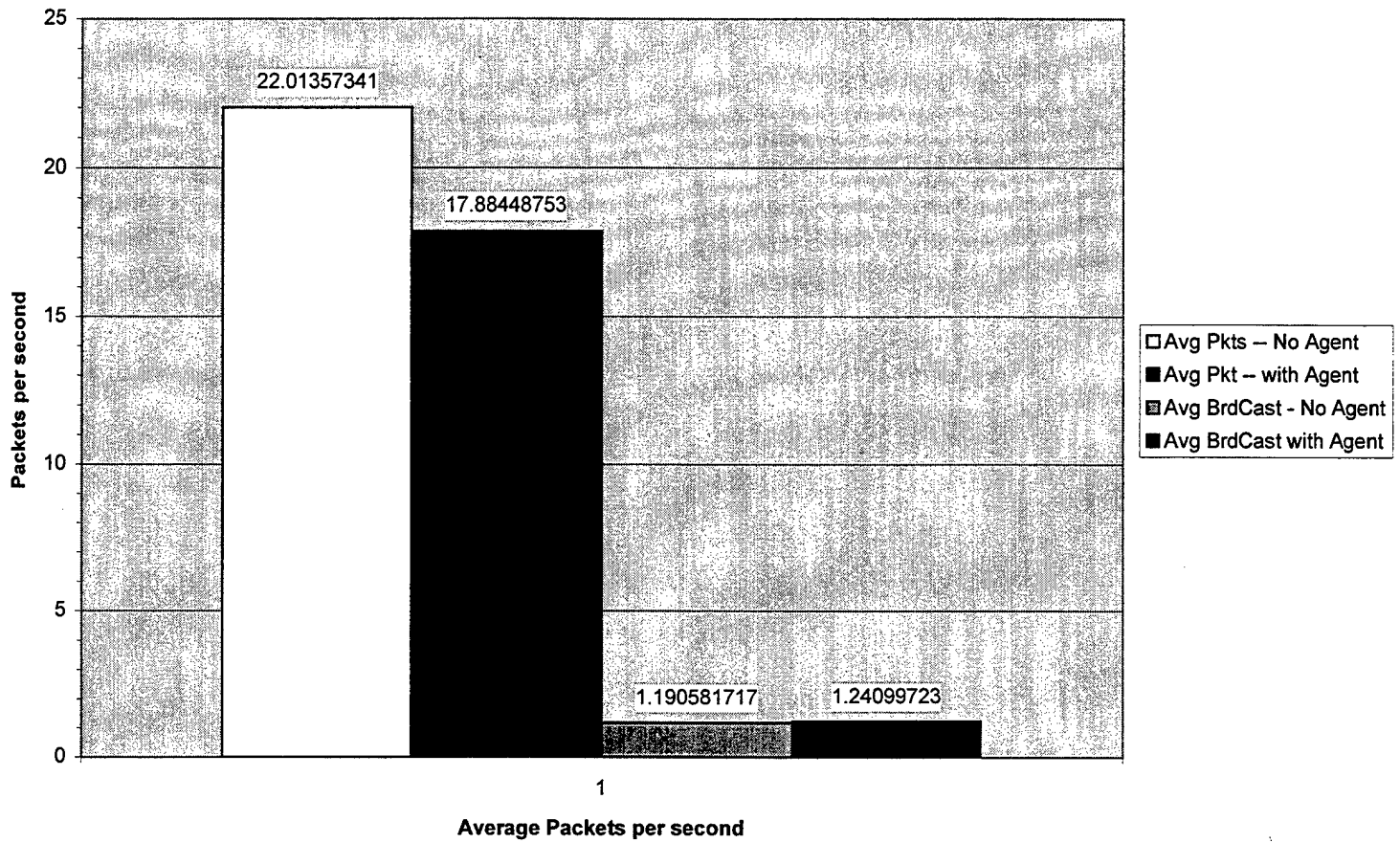
Figure 6: Average Packets and Broadcasts
