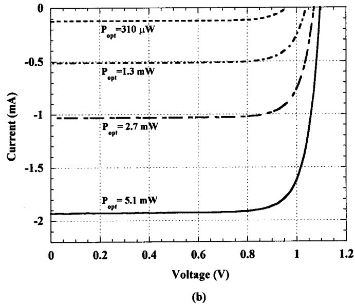
Figure 2.18: I-V curves as a function of illumination for single large area PV cells fabricated on a) oxidized wafer b) control wafer
