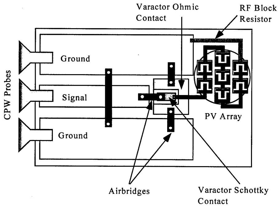
Figure 3.1: (a) Components of the monolithic OVC (b) Layout of the monolithic OVC.
