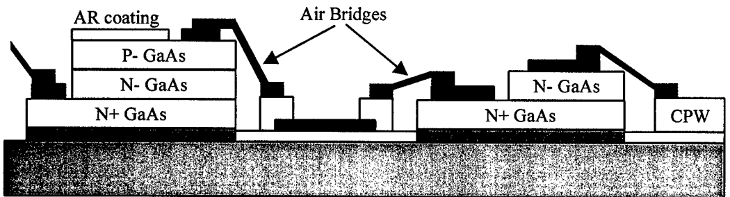
(h) Air bridge interconnections
