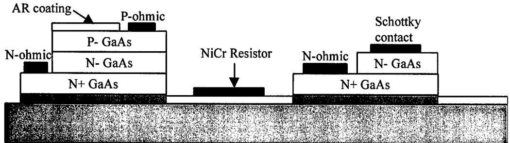
(f) AR coating and NiCr resistors
