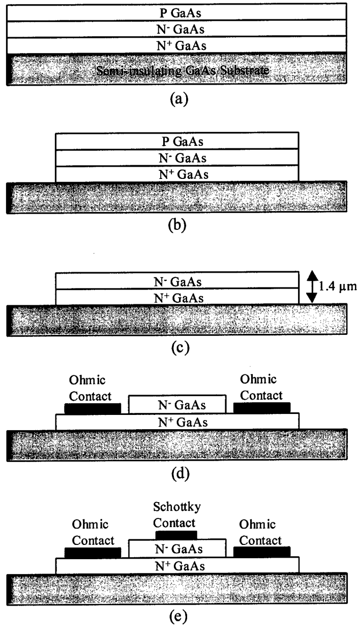
Figure 2.3: Fabrication process for the planar GaAs Schottky diodes
