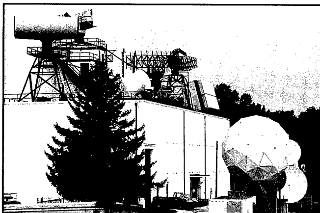
Radar test site at Building 75, Chesapeake Bay Section (Chesapeake Beach, MD) showing radar antennas used in experimental development by the Radar Division. On the roof, from left to right: experimental 3-D elevation phase scanned antenna for SENRAD, an experimental L-Band system; a directed mirror antenna (DMAR); and antennas for the SPS-49, SPS-10, IFF, SPS-40, and the fixed array surveillance radar (FASR). On the ground from left to right are antennas for: SPQ-9B advanced development model (in radome); a high resolution X-band clutter radar; and the high range resolution monopulse (HRRM) system.
