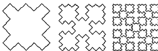
Sierpinski L-System surface filling fractal
