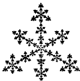
An IFS generated fractal snowflake Generated with FractalWorks 3.0 Lewin, 1997
