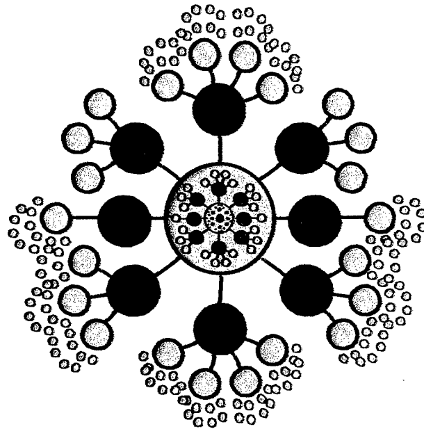
FractalSphere Drawing by Darren Gonski
