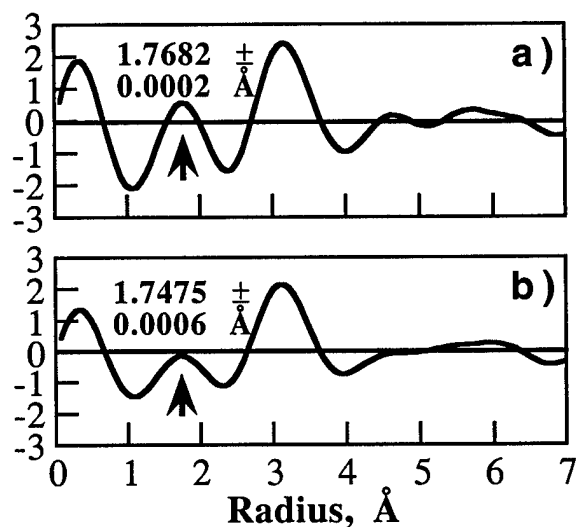
Figure 3. The reduced correlation functions 4\pi r(\rho(r) - \rho_0) (atoms per \text{\AA}^2 ) resulting from asymmetric (a) and symmetric (b) GIXS of SiC on Si are shown. The plots correspond to the data sets in figure 1 (b). The average first nearest neighbor distance or interatomic spacing is indicated by the arrow.
