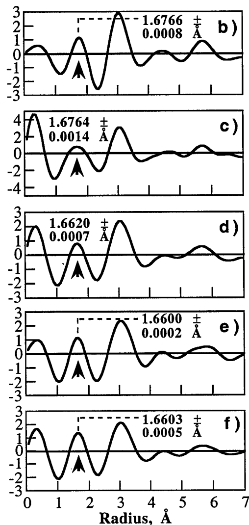
Figure 2. The reduced correlation functions 4\pi r(\rho(r)-\rho_0) (atoms per \text{\AA}^2 ) resulting from GIXS of \text{B}_4\text{C} on Si are shown. Figures (a) - (f) correspond to the six data sets in figure 1 (a) and to the first six experiments listed in Table I. Asymmetric mode results are in (a) - (c) while symmetric are in (d) - (f). In each figure, the average first nearest neighbor distance or interatomic spacing is indicated.
