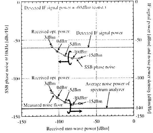
Fig. 5. SSB phase noise and noise power density (2)
