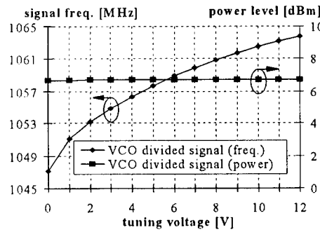
Fig. 7, Frequency and power dependence of the output signal of the digital divider
