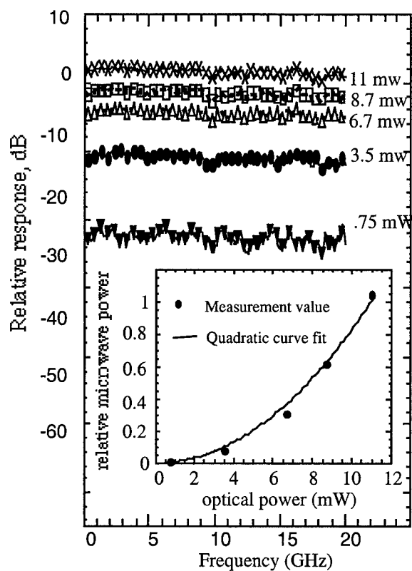
Fig. 2 Frequency response of photodetector A (30 \mu\text{m} long). The insert shows the quadratic relation between the microwave power and optical power.
