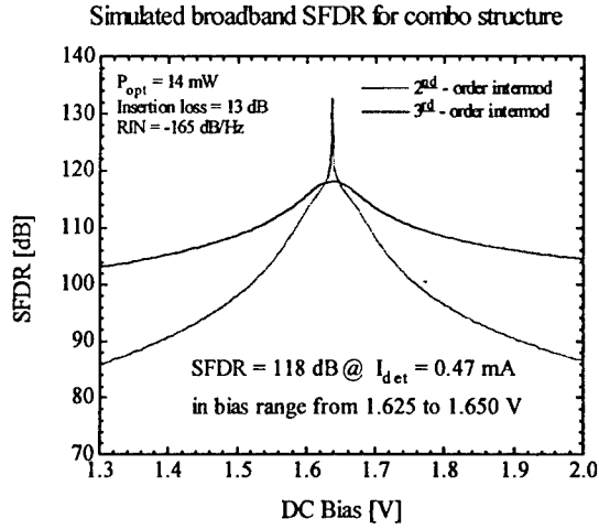
Fig. 6. Simulated SFDR in 1 Hz noise bandwidth of the DC transfer curve of Fig. 5, operating in TE polarization.
