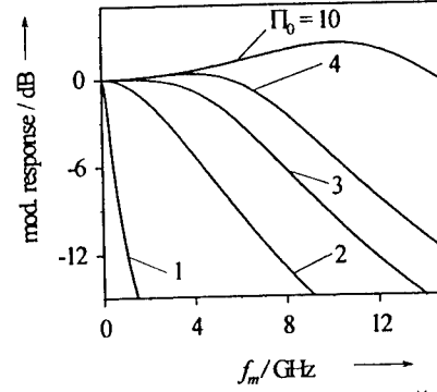
Fig 2. Small signal response 10 \log[\check{Z}_1(f)/\check{H}_1(f)]
