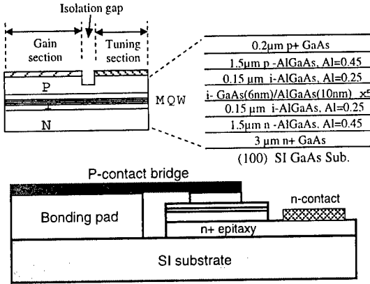
Fig.1 Structure of two-section QCSE tuned laser.
