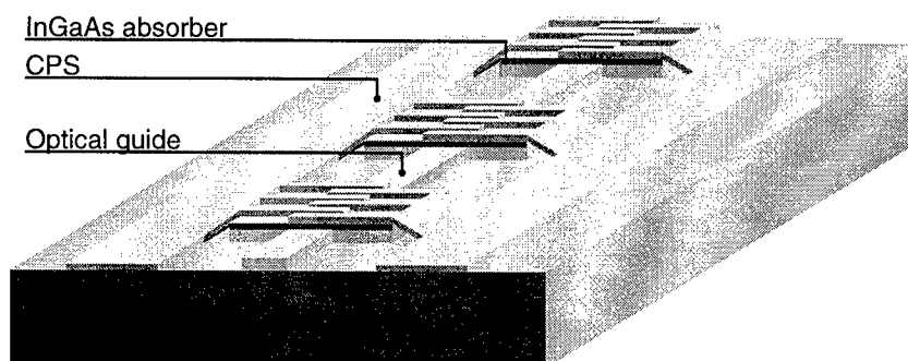
Figure 1: Schematic view of the distributed InGaAs MSM detector
