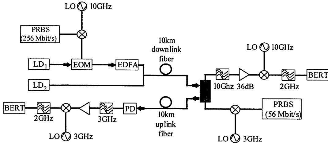
Fig. 2: Experimental set-up
