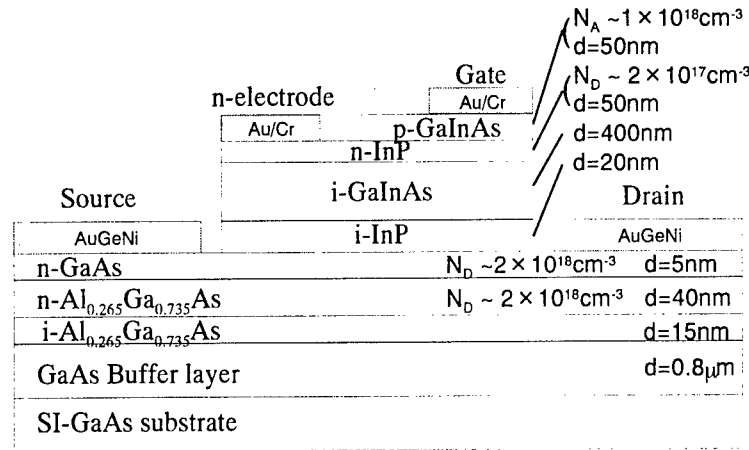
Fig. 1. Device Structure.
