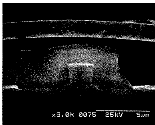
Fig. 1(b): Facet view of the device. A PMGI bridge is used to connect grounds from different sides of the waveguide.
