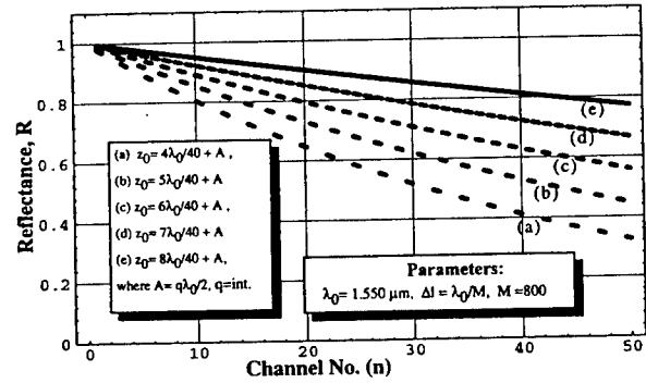
Fig. 2. The various reflectivity profiles R_n that can be coated onto M1 to obtain an increasing phase shift values for the reflected beamlets ( B_1 - B_n ) for different resonator spacing z_0 ( q is integer).
