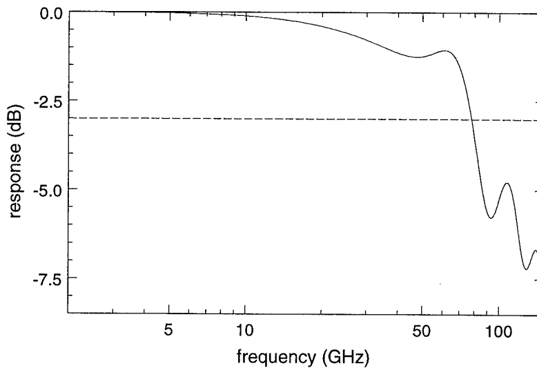
Figure 3: Corrected frequency response at 1.55- \mu m obtained from the pulse response shown in Fig. 2.
