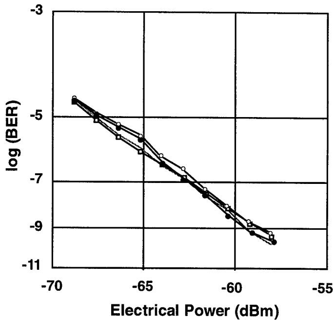
Fig. 2: Bit error rate vs. electrical power at the OQPSK receiver input. Modulation: 155 Mbit/s, PRBS. BER in CH1, CH2 without modulation( \bullet ). BER in CH2, CH1 without modulation(—). BER in CH1, both channels with modulation( \circ ). BER in CH2, both channels with modulation ( \square ).
