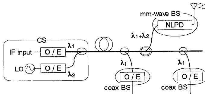
Fig. 3 Schematic diagram of a coax-wireless-hybrid fiber optic CATV system employing the nonlinear photo-detection scheme. The tow color optical carriers are utilized to feed optical IF and mm-wave LO signals.
