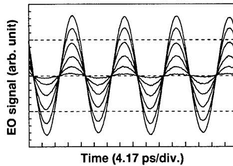
Fig. 6 Measured 60-GHz waveform for different photocurrents, 1, 5, 10, 15, 20, 25 mA.
