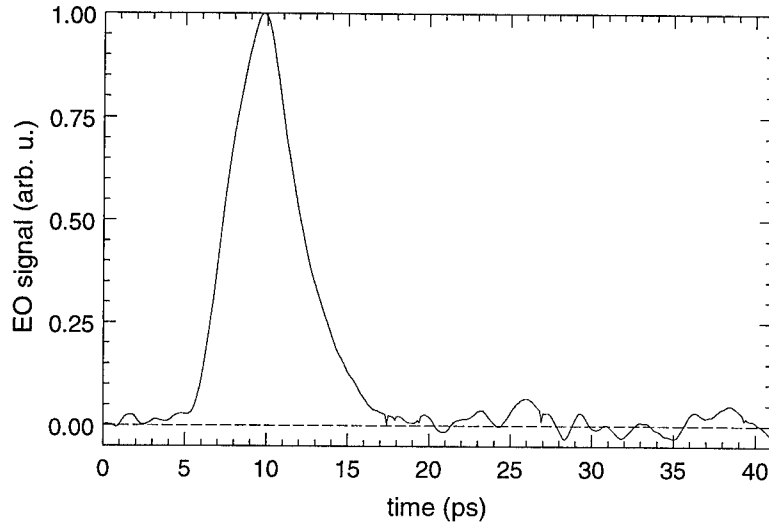
Figure 2: Pulse response at 1.55- \mu m light measured by electro-optical sampling.
