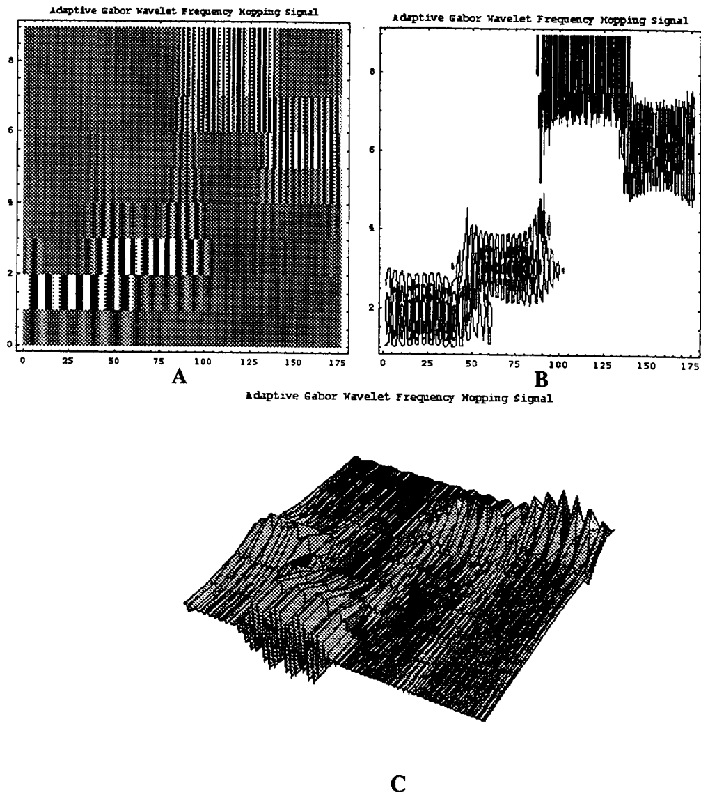
Fig. 8.6. Adaptive Gabor Representation of the frequency hopping signal with 6 x the bandwidth of the Gabor wavelet..
