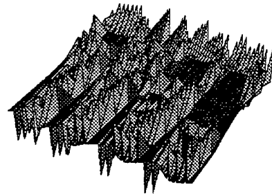
Differential Phase, 0th Order Gabor Wavelet, Frequency Mapping signal + Pulse
