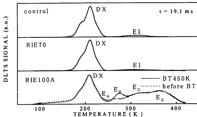
Fig. 4 DLTS spectra of the control, RIE70 and RIE100A samples. In the RIE100A sample, the spectrum after reverse bias temperature (BT) annealing at 450 K for 30 min is also shown.
