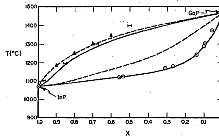
Figure 9. Equilibrium phase diagram for \text{In}_x\text{Ga}_{1-x}\text{P} . Taken from Ref. 14 and digitally edited.
