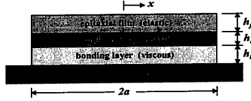
Figure 1. Schematic of a SOI compliant substrate system. The film and the compliant layer are treated as elastic membranes with deformation characterized by a longitudinal strain \epsilon = \partial u / \partial x . The bonding layer is a Newtonian viscous material which deforms in shear \gamma = \partial u / \partial y . In each case u is displacement in the x -direction.
