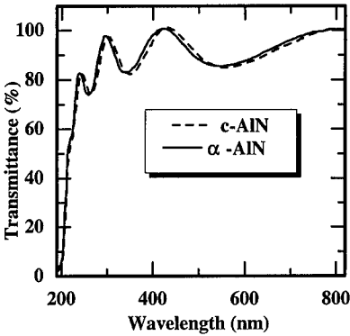
Fig. 4 Optical transmittance spectra of AlN thin films.
