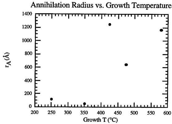
Figure 2. Experimental data for GaAs on InP system showing annihilation radii at various growth temperatures.
