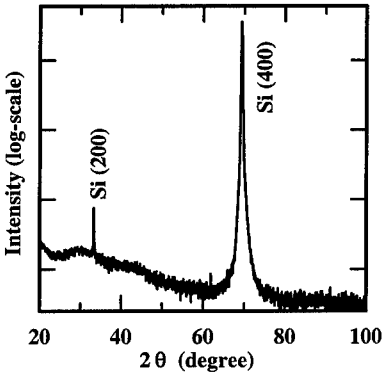
Fig. 2 XRD pattern of AlN thin films deposited at low temperature.
