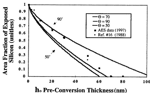
Figure 4: Predicted and measured thermal stability of thin GaAs/Si epitaxial films.
