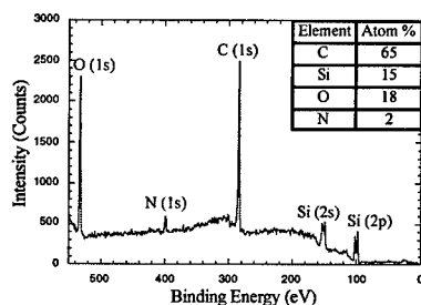
Figure 3: XPS spectrum of the wafer side fracture surface
