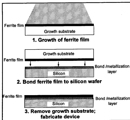
Figure 1. Fabrication steps for the integrated ferrite / silicon circulators.
