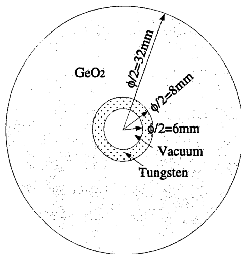
Figure 6. Configuration for calculating shock wave decay in spherical geometry. At time zero, tungsten core impacts surrounding GeO 2 at 1.5 hr/sec simulating impact at surface of a half-space.
