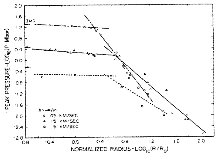
Figure 16. Log 10 (peak shock pressure) versus log 10 (normalized radius) at various impact velocities for gabbroic anorthosite impactors. Arrows indicate one-dimensional flow pressures. Close in region that has minor attenuation results from a quasi-planar flow (Regime A of Figure 17). Minor divergence of flow induces minor stress wave decay immediately beneath striking projectile (after Ahrens & O'Keefe 1977)
