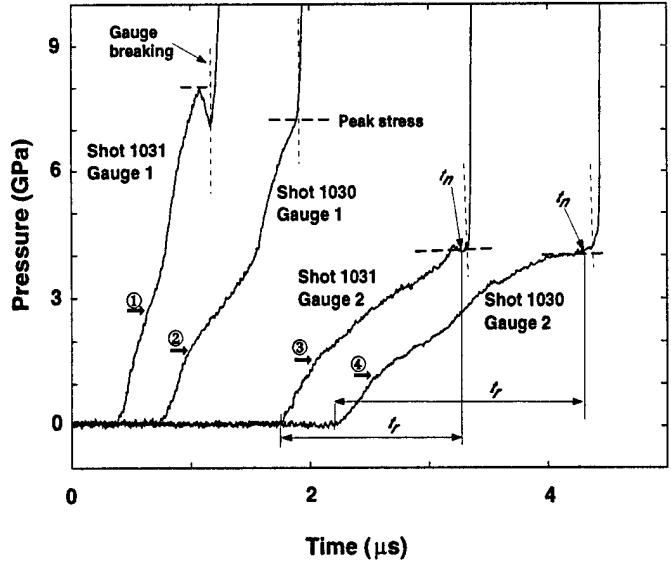
Figure 15. Stress-wave profiles for spherical impactor in vitreous GeO 2 . Arrows indicate the amplitude of the precursor originating from impact surface. Note the peak stress decays for 8 to 4 GPa over a 3 mm increment in radius.
