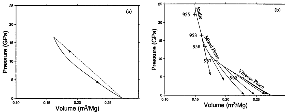
Figure 1. Hugoniot and release isentropes for: (a) reversible phase change models; (b) irreversible (several measured releases at different pressures are shown). For reversible model, release are not distinguishable from Hugoniot. "Waste heat" is area between the Rayleigh line (dashed) and the solid curve release isentrope induces normal attenuation. The hysteretic behavior of Hugoniot-release isentrope loop in (b) enhances dissipation of shock energy and gives rise to increased attenuation.
