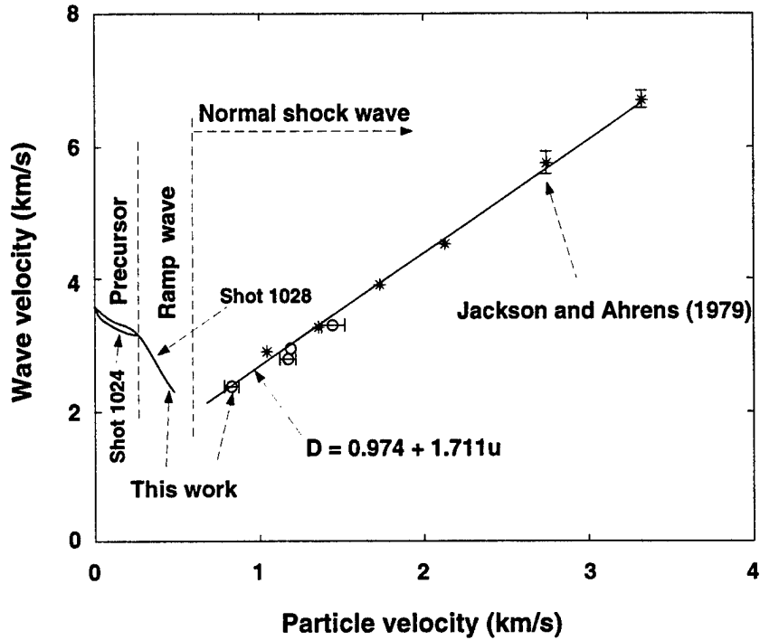
Figure 3. Shock wave versus particle velocity, vitreous GeO 2 , initial density.
