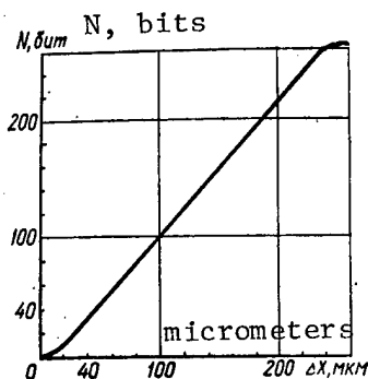
Figure 2. Graph of the conversion characteristic of the transducer with the A/D converter.
