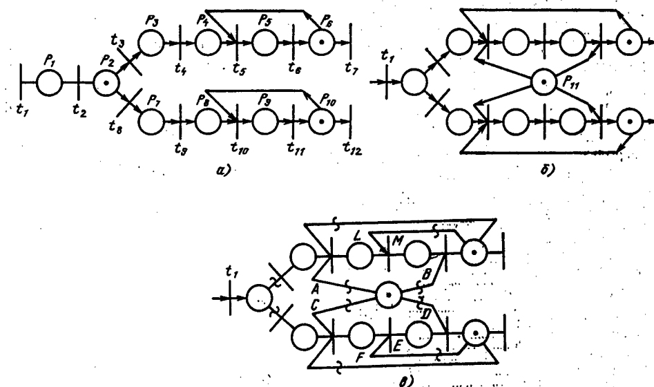
Figure 2. Representation of operation of transport vehicles by a Petri net.
