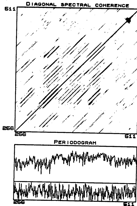
Figure 7: (Top) Spectral coherence image from XC5.7 time series. Starting time: 69,520 samples. N=8192 , M=32 . Frequencies shown are in the range .003125F_s , .006238F_s . (Bottom) Periodogram of the same data for same frequency band with N=8192 .
