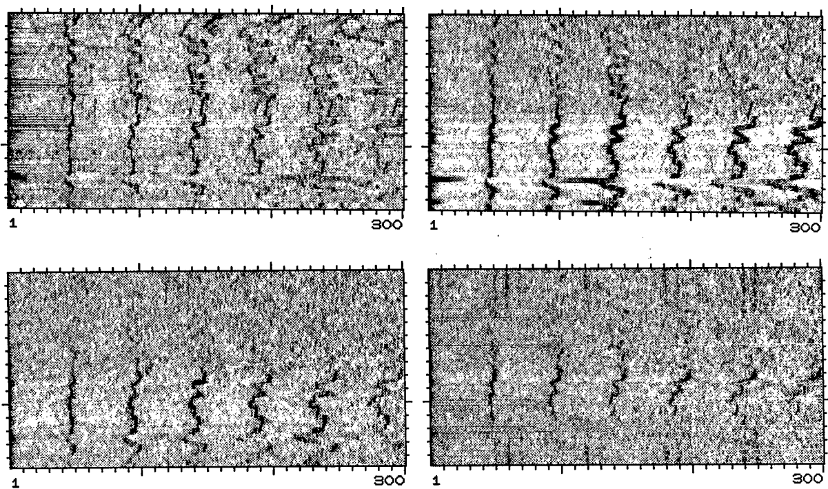
Figure 11: Average coherence grams of data GV9A1060; FFTLEN=2048; SLIDE=1024. (Top left) xBins=[1:512], yBins=[1:512]. (Top right) xBins=[513:1024], yBins=[513:1024]. (Bottom left) xBins=[1025:1536], yBins=[1025:1536]. (Bottom right) xBins=[1537:2048], yBins=[1537:2048].
