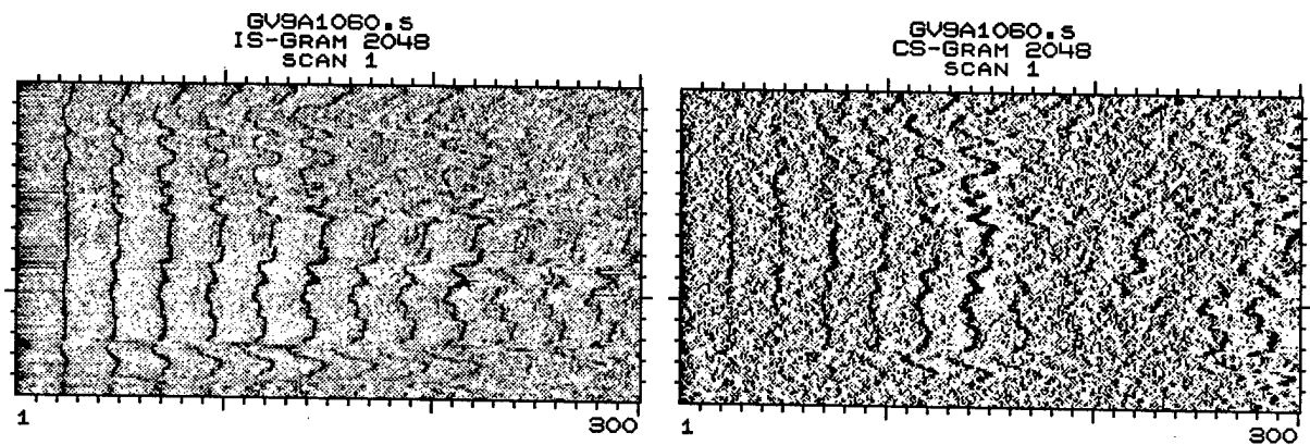
Figure 10: (Left) Average coherence gram of data GV9A1060; FFTLEN=2048; SLIDE=1024; xBins=[513:1024], yBins=[513:1024]. (Right) Squares spectrogram of data GV9A1060; FFTLEN=2048; SLIDE=1024.
