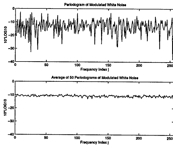
Figure 2: (Top) Periodogram of X(t) = f(t) \cdot Y(t) with f(t) = f(t + 32) and f(t) = 0 or 1 according to Eq. (5). N = 512 . The frequency corresponding to the index j is \lambda_j = 2\pi j/N . (Bottom) Average of 50 independent periodograms of the same series.
