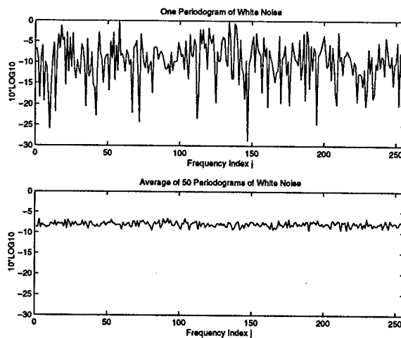
Figure 3: (Top) Periodogram of white noise X(t) . N = 512 . The frequency corresponding to the index j is \lambda_j = 2\pi j/N . (Bottom) Average of 50 independent periodograms of the same series.
