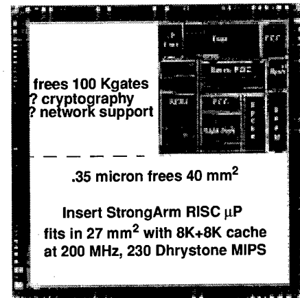
(b) Next-generation ASIC (0.35 micron technology)
