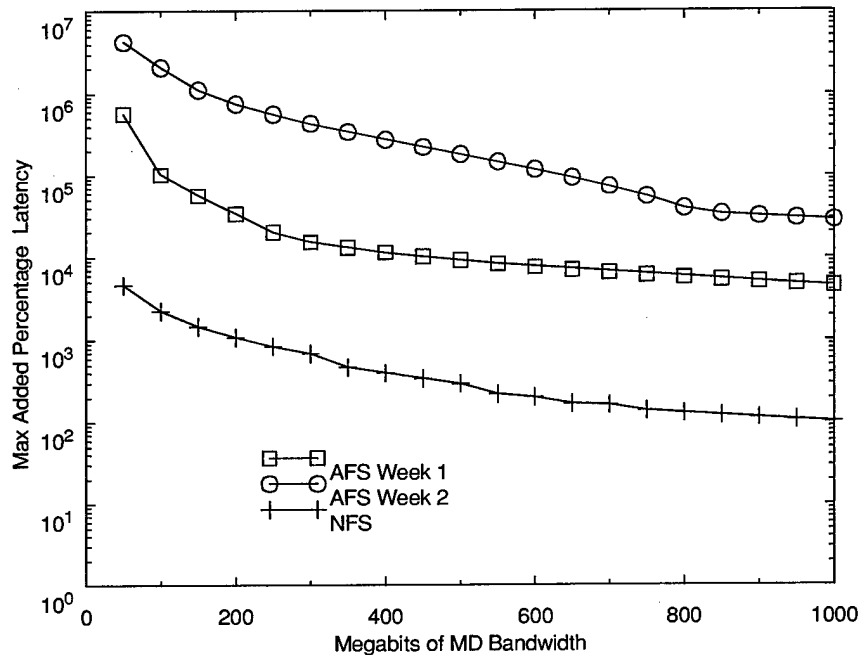
Figure 7-8 Maximum Additional Latency Seen by Clients
