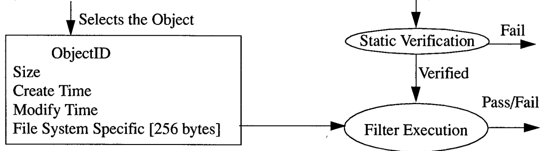
Figure 5-7 Evaluation of a Metadata Filter Credential
