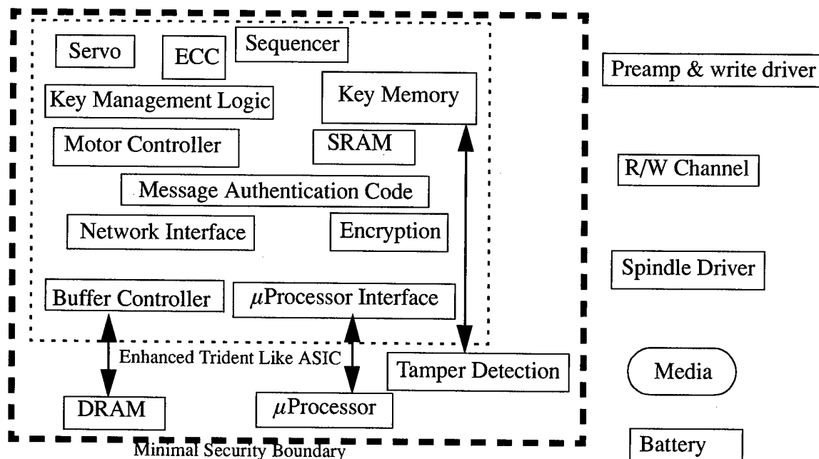
Figure 8-2 Security Boundary in a Viking Like Implementation
