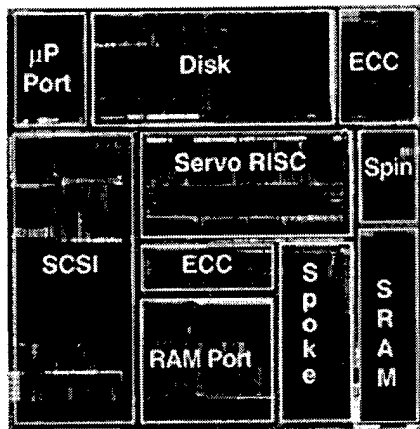
(a) Current Trident ASIC (74 mm 2 at 0.68 micron)
