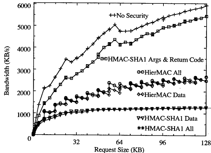
Figure 6-3 HierMAC Performance
