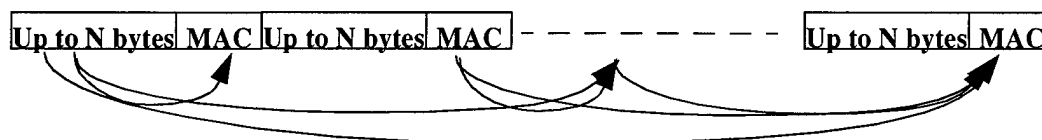
Figure 6-11 Inline Message Authentication Codes
