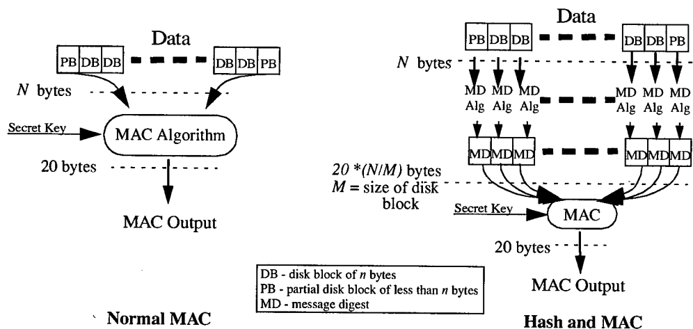
Figure 6-2 MAC Structures
