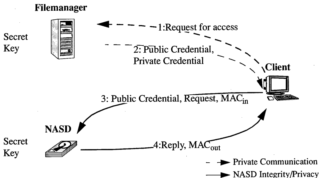
Figure 4-2 Overview of NASD Security
