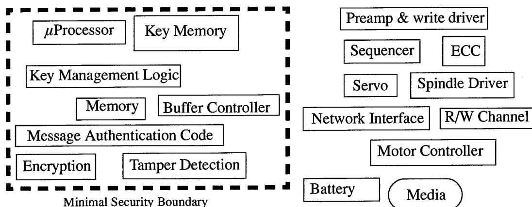
Figure 8-1 Minimal Security Boundary
