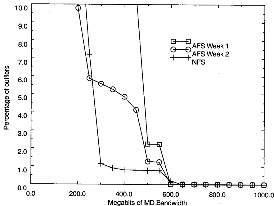
Figure 7-7 Percentage Outliers
