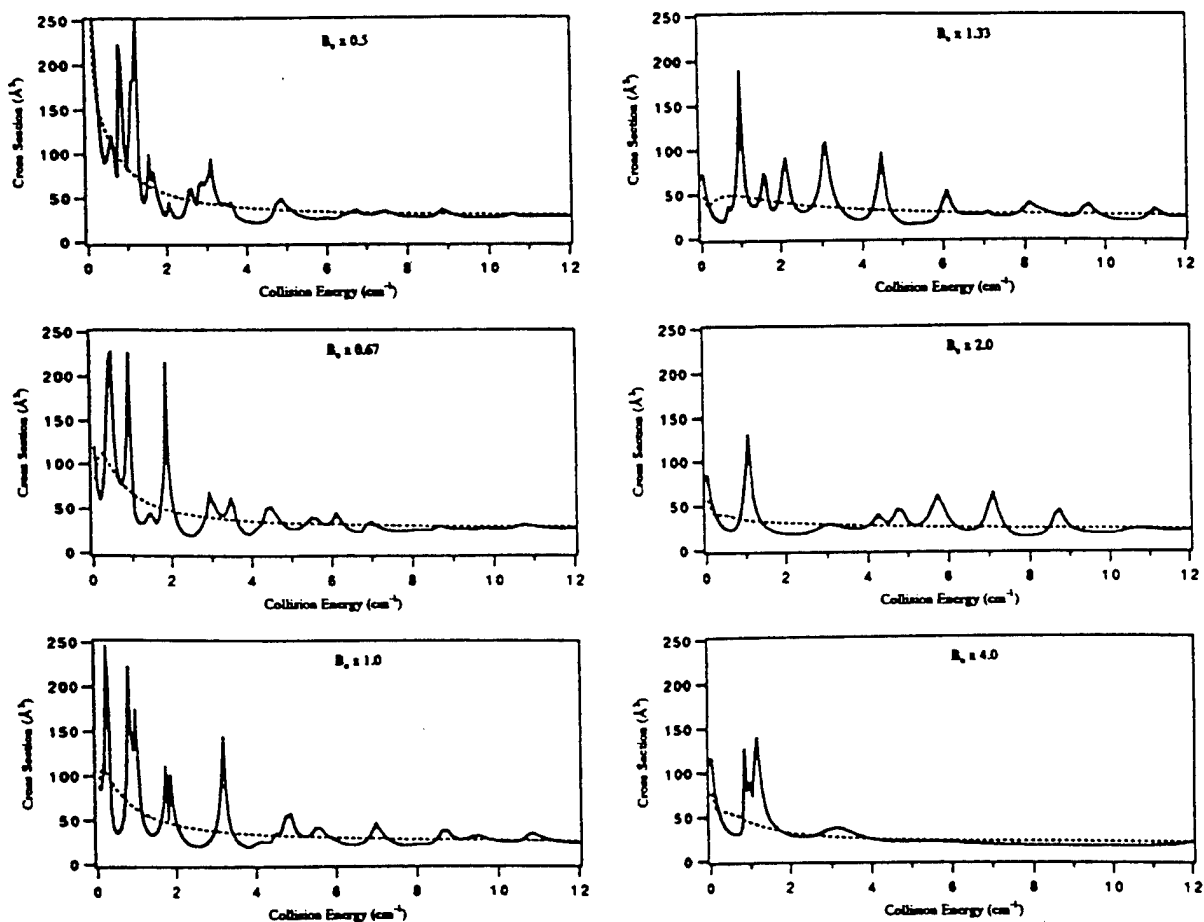
Figure III.A.7. Calculated pressure broadening cross sections for the J = 0 - 1 line of CO. The smooth lines represent the thermal average with T(K) = 1.5 E (\text{cm}^{-1}) .
