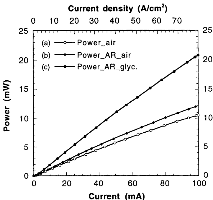
Figure 7: Light output versus current characteristic of a 400 \mu\text{m} diameter diode (a) without anti-reflection coating into air, (b) with anti-reflection into air and (c) with anti-reflection coating into glycerine.
