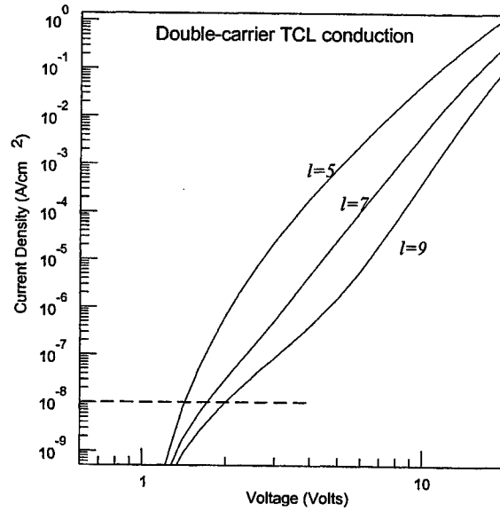
Fig. 1. Calculated TCL current-voltage ( J - V ) characteristics for three l values ( l=5, 7, \text{ and } 9 ). Power law dependence ( J\sim V^{l+1} ) is obtained. The horizontal dashed line at J=10^{-8} \text{ A/cm}^2 illustrates the experimentally observed background current. The parameters we used for this simulation are: H_p=H_n=10^{19} \text{ cm}^{-3} , T=300\text{K} , \epsilon_r=3.4 , n_i=1 \text{ cm}^{-3} , E_g=2.4 \text{ eV} , K_b=10^{-4} \text{ cm}^3/\text{s} , \mu_n=5\times 10^{-5} \text{ cm}^2/\text{V}\cdot\text{s} , \mu_p=0.01\mu_n , n_o=p_o=\rho_o=5\times 10^{20} \text{ cm}^{-2} , L=60\text{nm} . See the parameter definitions in Ref. [14].
