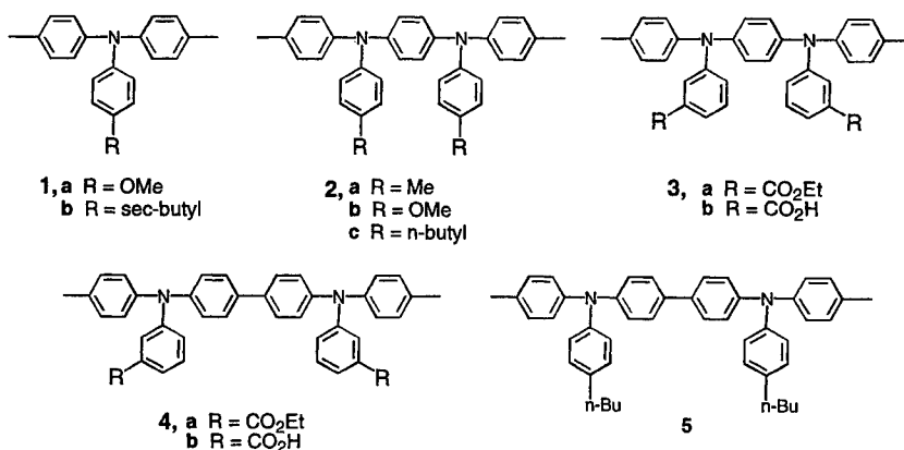
Figure 5. Aromatic Amine comonomers in fluorene alternating copolymers.
