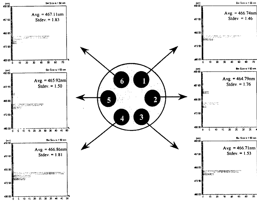
Fig.7 : PL wavelength uniformity from a blue LED run. All six wafers have tight distribution of wavelength with standard deviation better than 2 nm
