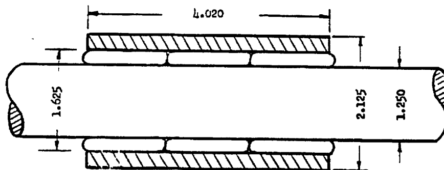
Figure 2. Track Bushing Assembly.
