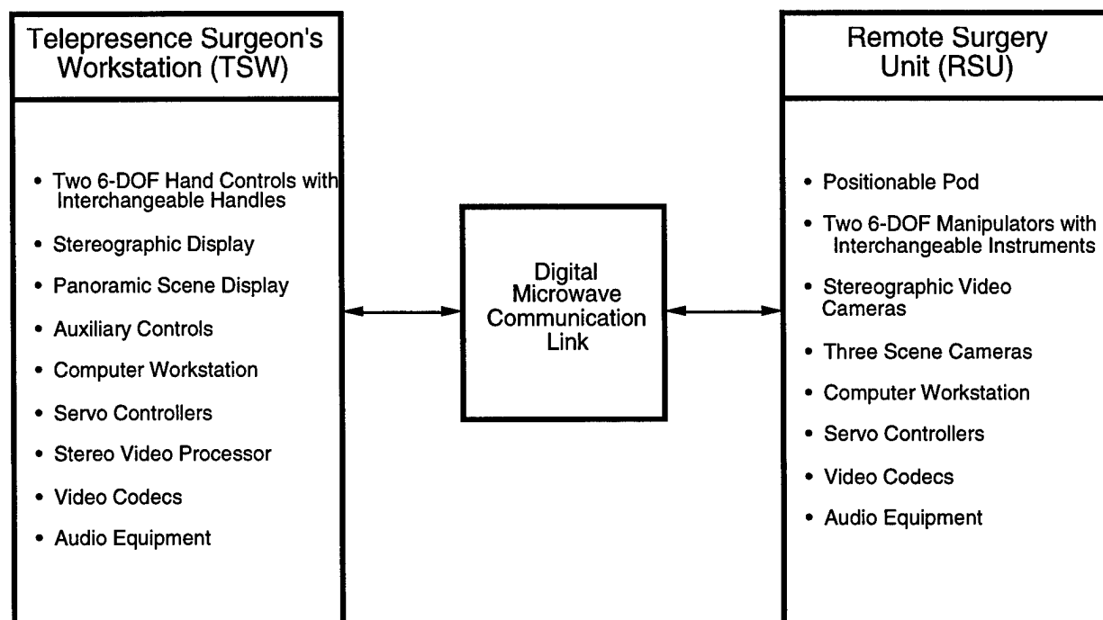
Figure 2. MEDFAST system block diagram. The complete MEDFAST system consists of the telepresence surgeon's workstation, the communication link, the remote surgery unit, and electronics modules associated with the TSW and RSU.
