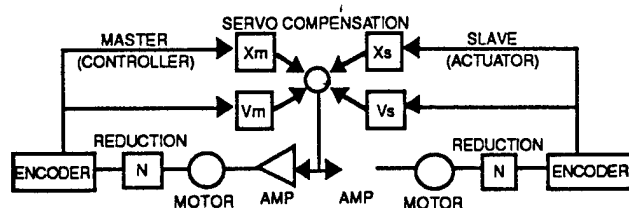
Figure 7. Manipulator Control Diagram
