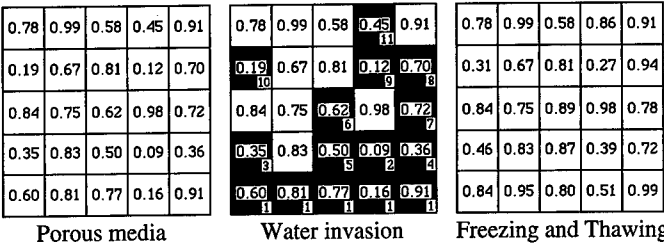
Figure 3 - Illustration of the invasion-freezing process: (i) a 5x5 lattice representing the porous material, (ii) the invasion of the porous material by a fluid (represented in dark), the labels give the evolution of this invasion, and (iii) the porous structure after the freezing process.
