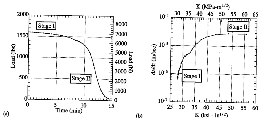
Fig. 5. (a) Load relaxation due to cracking in IN718 in lab air for a SEN specimen loaded to a fixed displacement at 650°C. (b) Corresponding v-K curve. Ref. 11.
