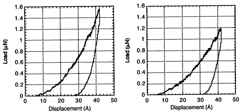
Figure 1. Load-displacement curves for (a) \alpha -Si 3 N 4 and (b) amorphous Si 3 N 4 .
