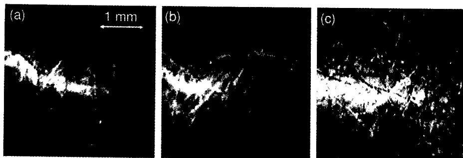
Figure 4. Damage shown with the light shades of gray in mixtures of PGW and softwood kraft (black) in SENT. The mass fraction of kraft fibers is 5% (a), 10% (b) and 20% (c).
