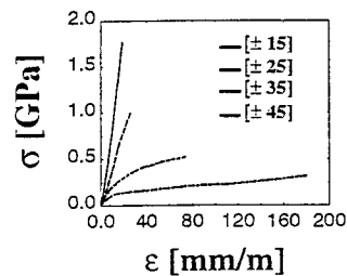
Figure 2: Strength-deformation diagram for different fibre inclinations. The samples with fibre's angulation of 35 and 45 degrees have non-linear behaviour.
