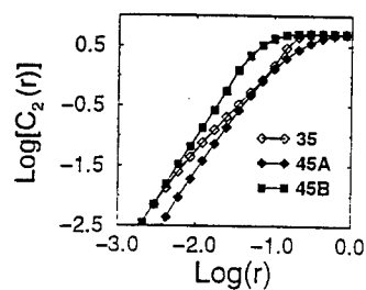
Figure 7: Scaling of the correlation integral vs. r . The fractal dimension is the slope of the function. We found respectively D_2 = 1.51, 1.35, 1.35 for 35, 45A, 45B.
