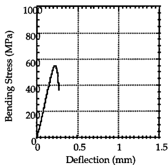
Figure 6: Crosshead disp. rate = 0.1 mm/min; T = 686^{\circ}\text{C}
