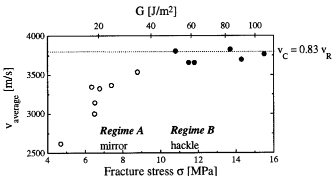
Fig. 3: Average crack velocity for the (110)[1\bar{1}0] crack system as a function of the far-field stress at the onset of fracture. An increase of the velocity at lower stresses is followed by a regime where the velocity curve saturates. The generated fracture surface is smooth and mirror-like over the whole crack path (open circles) for the lower stresses. At high stresses a transition from mirror to hackle zones is observed along the crack propagation direction (solid circles).
