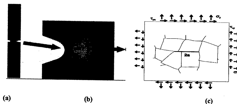
Fig. 1: Meso-macro connection, a) specimen, b) enlarged FEM net, c) boundary stresses for the simulation
