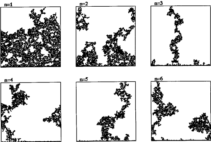
Figure 4 - Successive percolating clusters observed on a 200x200 lattice after n=1,2,3,4,5 and 6 iterations.
