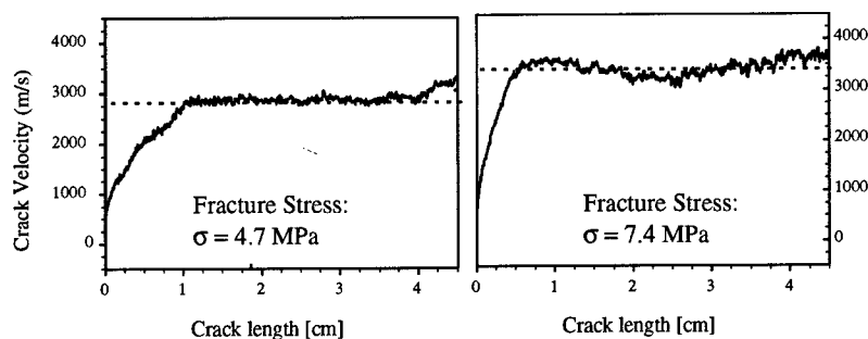
Fig. 2: Crack velocity as a function of the crack length for two specimens which were fractured on a (110)[1\bar{1}0] cleavage system. After an initial acceleration period the crack propagates at a steady velocity which depends on the applied far-field fracture stress.
