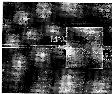
Figure 3. SEM image of the failure location.
