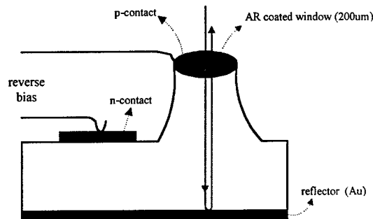
Figure 2.2: A Schematic of the PIN structure used to measure the photocurrent spectra of the MQW wafer MR1074. The device diameter is 200 \mu\text{m} for ease of optical access in the measurement arrangement.
