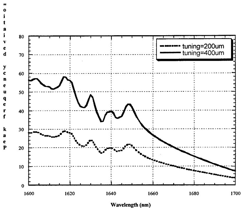
Figure 2.7: The maximum frequency deviation as a function of wavelength for an 800 μm long laser with tuning section lengths of 200 and 400 μm respectively. The bias level is assumed to be -3V with \Gamma = 0.1 .
