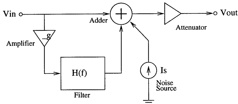
Figure 3.2: A schematic of the equivalent circuit representing the optical gain within a subsection.
