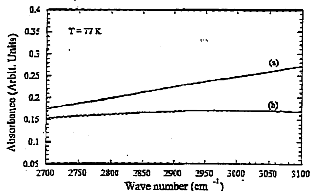
FIG. 4. Absorbance spectra of samples K [spectrum (a)] and L [spectrum (b)]
