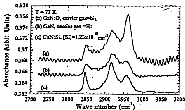
FIG. 2. Carbon-hydrogen localized vibrational mode spectra of GaN samples E, F, and G measured at 77 K. Spectra (a), (b), and (c) were obtained for undoped but O_2 contaminated sample (E), undoped sample (F)
