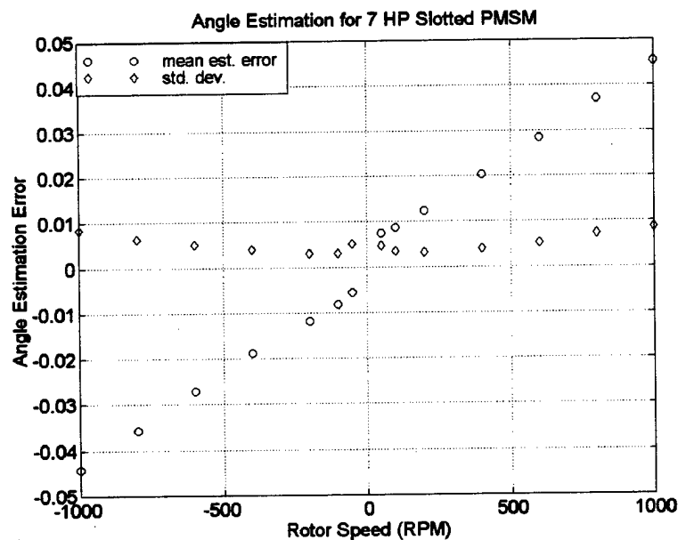
Fig. 21 Rotor position estimation accuracy of slotted PMSM using direct phase voltage measurement
