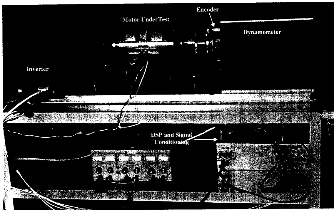
Fig. 16 Experimental setup for sensorless drive
