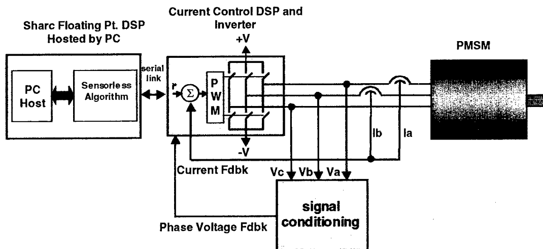
Fig. 19. Block diagram of experimental system
