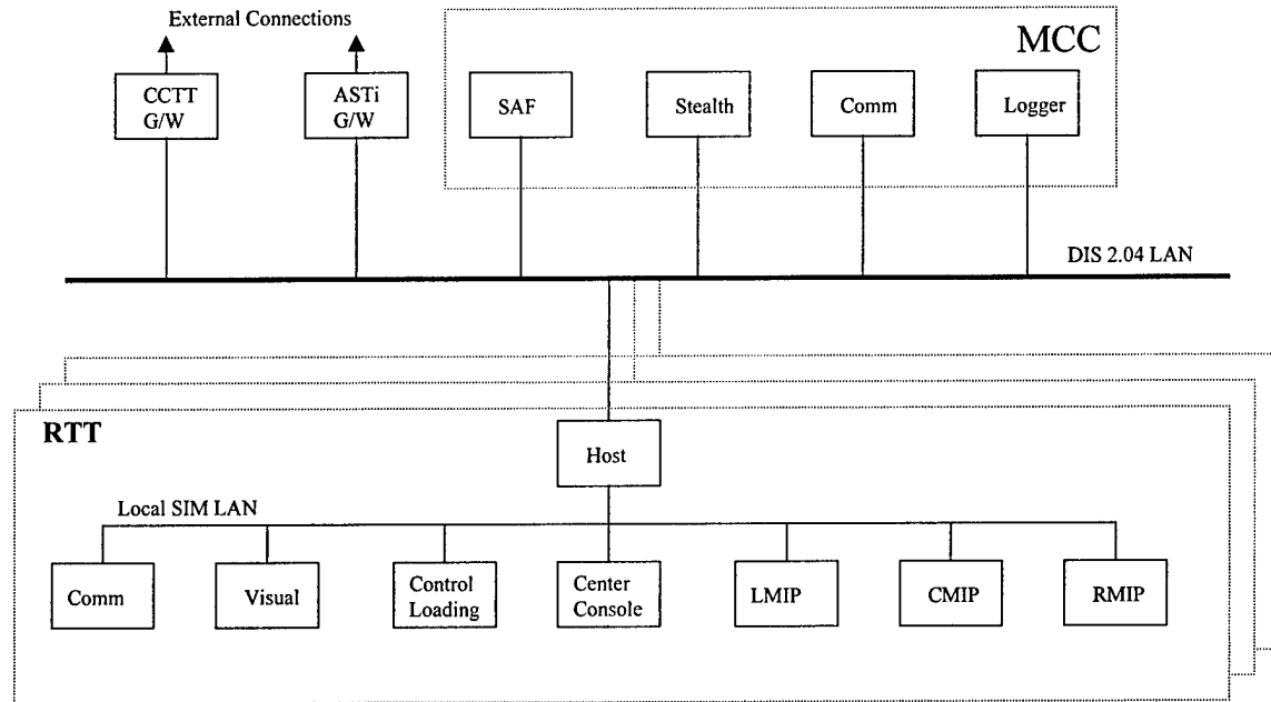
Figure 3-4. Network Architecture
