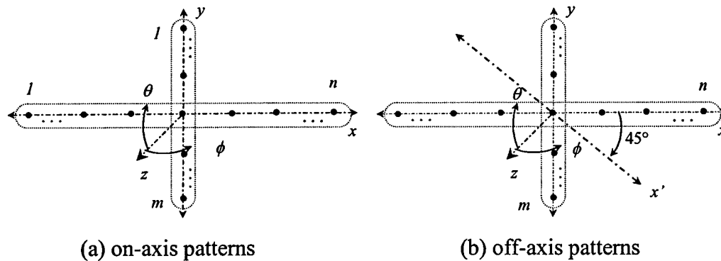
Figure 6.3-22. Equivalent Array of Sources for Patterns in x - and y -directions.
