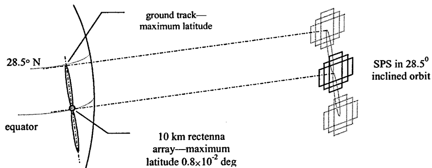
Figure 7.2-18. Effect of Orbit Inclination on Beam Steering for GEO SPS.
