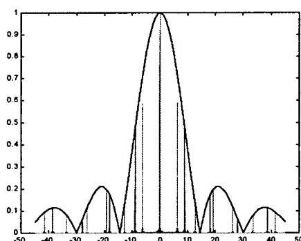
Figure 7.3-8. Comparison of Diagonal and Lateral Beam Patterns at Broadside.
