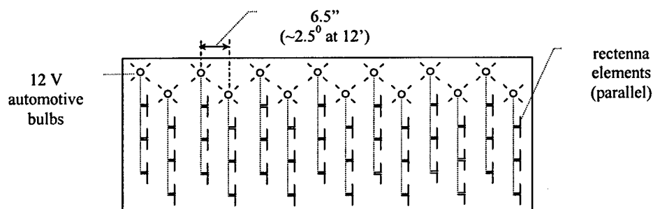
Figure 6.4-5. Rectenna Indicator Panel Layout.
