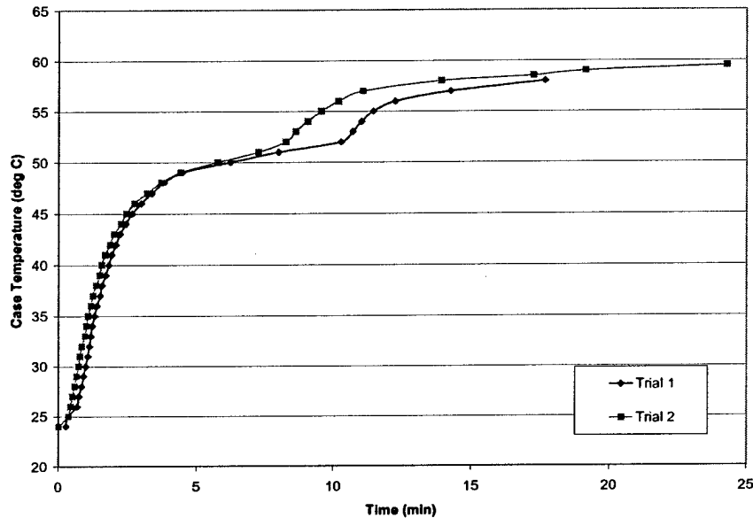
Figure A.4.6-1. Warming Curve for Hitachi 2M170 Magnetron.
