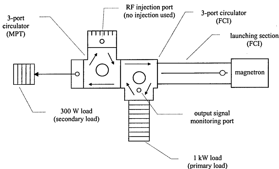
Figure 3.1-4. Primary Test Configuration for Magnetron.
