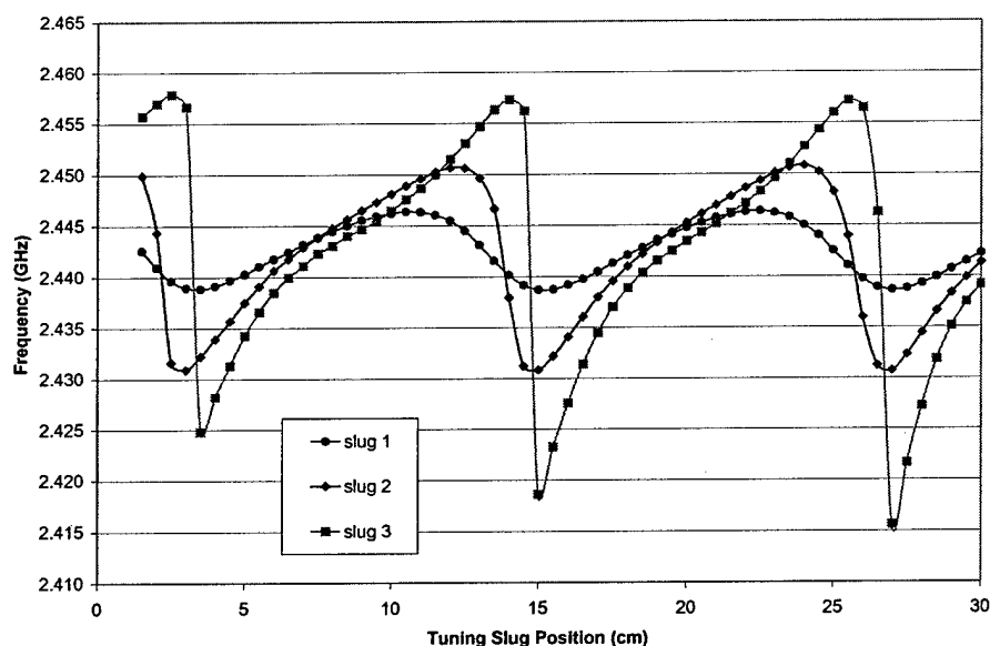
Figure 5.4-1. Effects of Tuning Slug Location on Operating Frequency for a Class II MDA. Larger slugs produce greater frequency pulling range.
