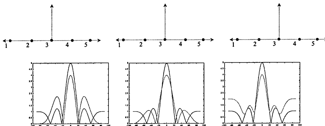
Figure 6.3-19. Effect of Missing Elements on Linear Array of Point Sources. Curves not normalized to emphasize effect on pattern gain.
