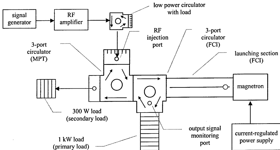
Figure 3.3-3. Physical Configuration of a Class II MDA.
