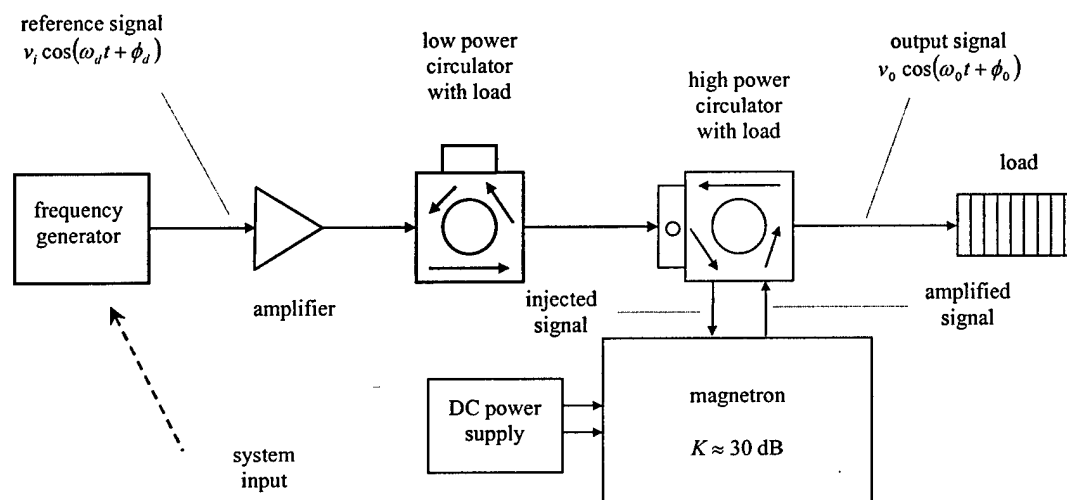
Figure 3.2-1. Class I MDA Functional Diagram. Frequency generator is the only system input.
