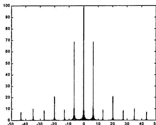
Figure 6.3-28. Diagonal Pattern for 100-Element Array of SWA Antennas, S_\lambda = 6.17\lambda . Blue (dark) line shows 100 element diagonal; green (light): 70 elements.
