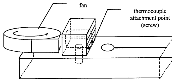
Figure 3.1-5. Measurement Scheme for Magnetron Temperature.
