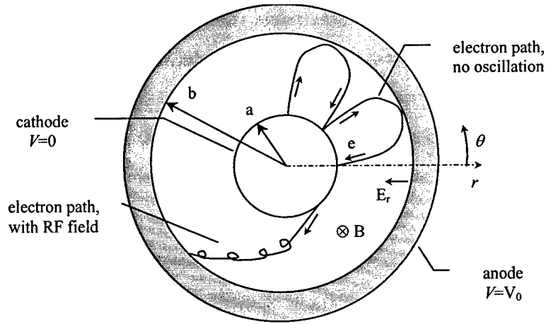
Figure 4.1-2. Simplified Magnetron Cavity. Cathode has radius a and anode radius b . Electron path shown before and during oscillation [15], [16].
