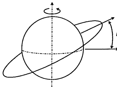
Figure 7.2-12. Measurement of Orbit Inclination.
