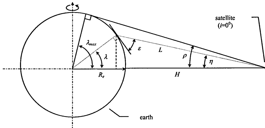
Figure 7.2-1. Earth Angular Geometry for SPS [25].
