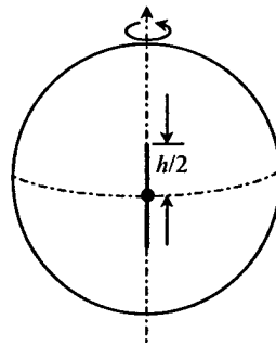
Figure 7.2-13. Periodic Motion of GEO Satellite Due to Orbit Inclination. Differential rotation rate due to earth latitude neglected.
