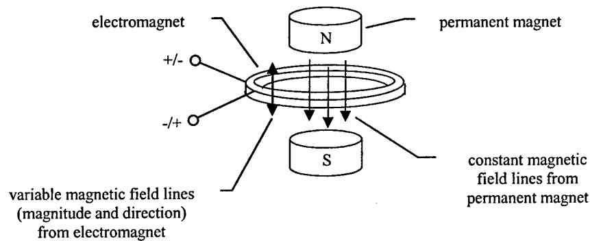
Figure 3.6-2. Magnetic Flux Lines from Permanent Magnets & Electromagnet.
