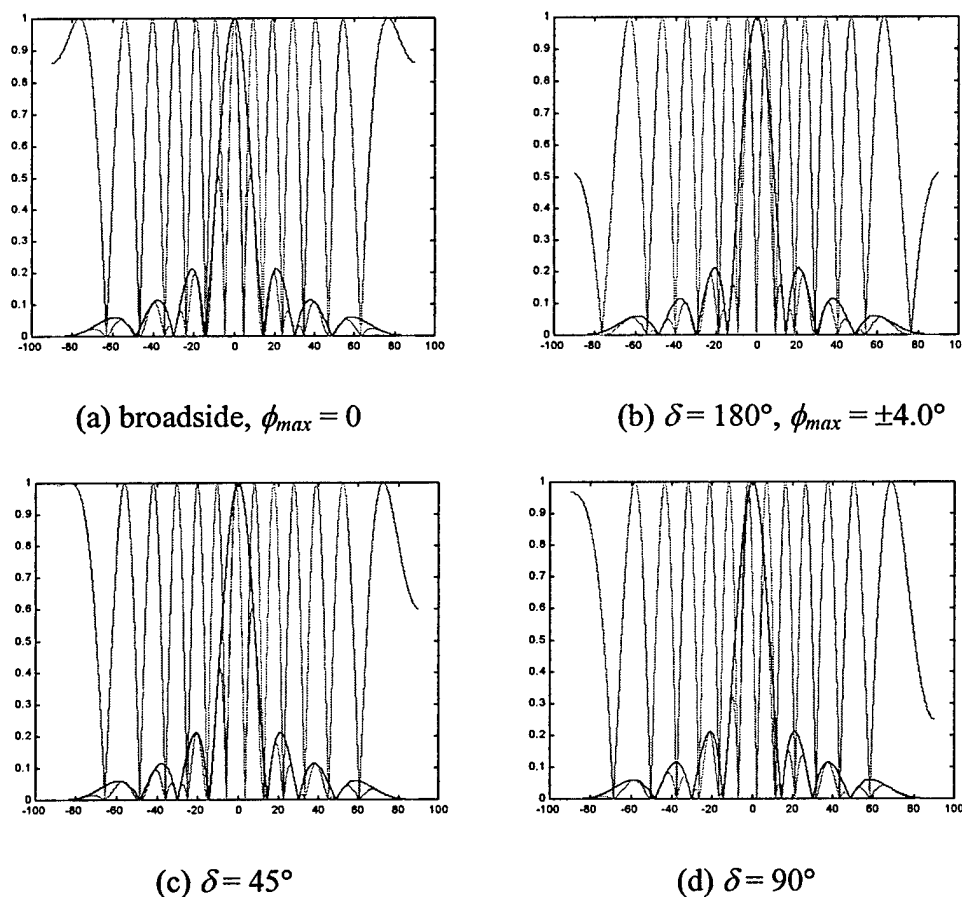
Figure 6.3-18. Pattern Decomposition for 2-Element Array of SWA Antennas.
