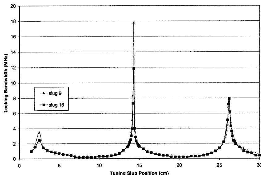
Figure 5.4-20. Locking Bandwidth Using Reactance Tuning Slug and Injected Reference Signal for a Class III MDA. Data shown for slugs 9 and 16.
