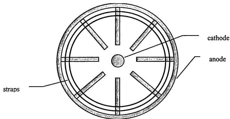
Figure 4.1-1. Cross-Section of a Strapped Magnetron [15].
