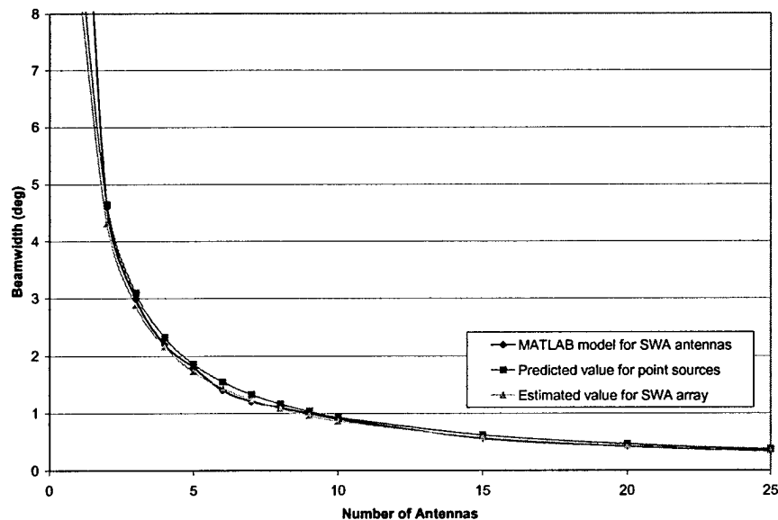
Figure 6.3-8. Resultant 3 dB Beamwidth versus Number of Sources.
