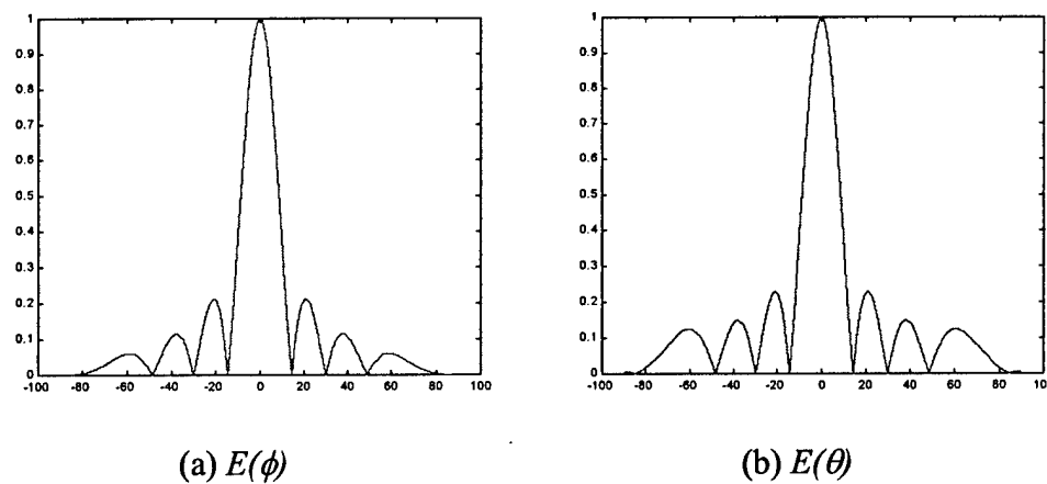
Figure 6.2-4. Fringe Plots of E -fields for 64-Element Slotted Waveguide Array.
