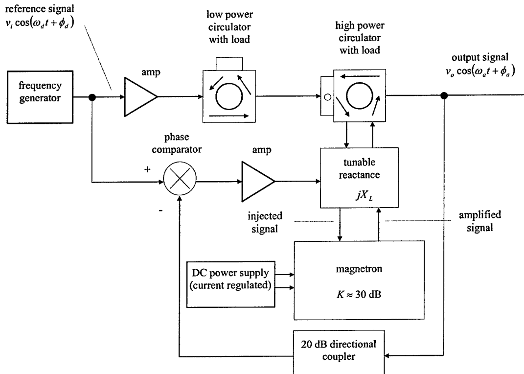
Figure 3.5-1. Class III CL MDA Functional Diagram.
