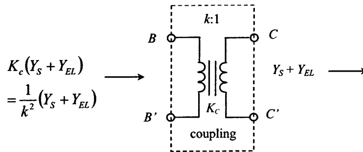
Figure A.4.3-7. Transformer Model for Magnetron RF Probe.
