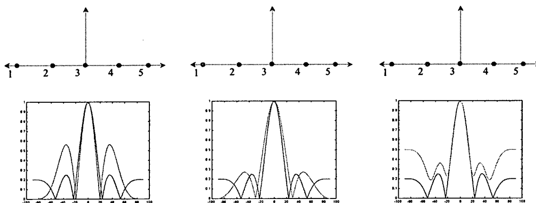
Figure A.1.2-4. Effect of Missing Elements on Linear Array of Point Sources.
