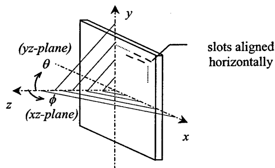
Figure 6.2-1. Geometry for Beam Measurements of Slotted Waveguide Array.
