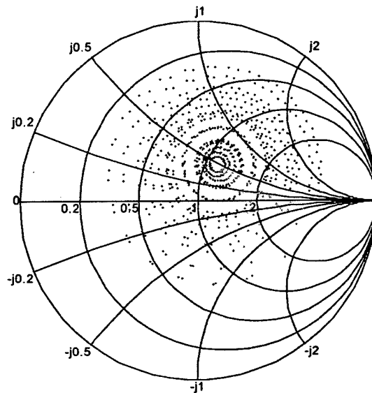
Figure A.4.1-6. Set of all MDA Load Impedances. Light blue points indicate general region of 'sink' for Rieke diagram.
