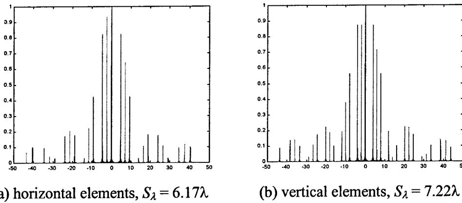
Figure 7.3-3. Patterns for 530 x 450 Elements SWA Antennas. Blue lines depict no phase shift; orange: 90° shift; red: 180° shift.
