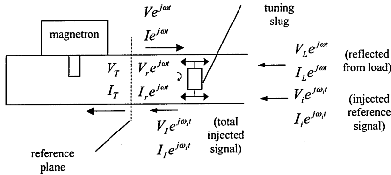
Figure 4.2-2. Magnetron-Load Interface (Transmission Line Equivalent).
