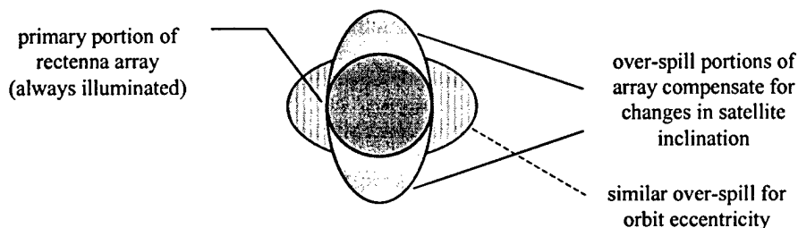
Figure 7.2-19. Effects of Satellite Inclination on Rectenna Array Shape. Assumes beam is dynamically directed to array center.
