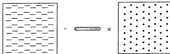
Figure A.1.1-3. Graphical Equivalent of Pattern Multiplication for SWA.
