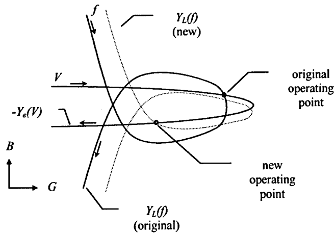
Figure A.4.6-4. Intersection of Load and Electronic Admittance Curves [15].
