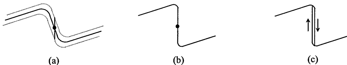
Figure 5.4-15. Effect of Frequency Curve Shape on Locking Bandwidth. (a) BW limited by slope of curve, (b) full BW available, (c) no BW available.
