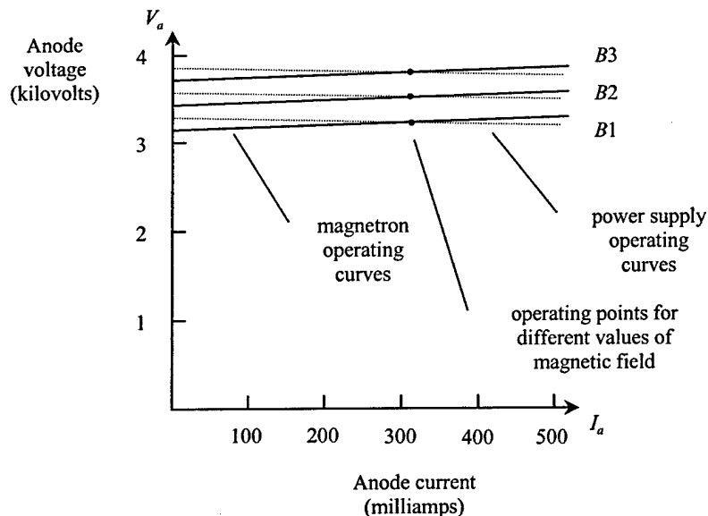
Figure 3.3-2. V - I Characteristic Curve for Magnetron.
