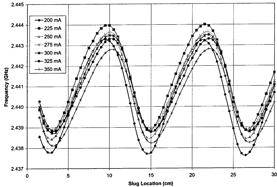
Figure 5.4-28. Effect of Power Control on Frequency Response for a Class III MDA, Slug 1. Chart intended to illustrate chaos of curves. An expended scale chart is shown in Figure 5.4-29.
