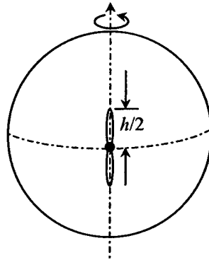
Figure 7.2-14. Ground Track of GEO Satellite Due to Orbit Inclination.
