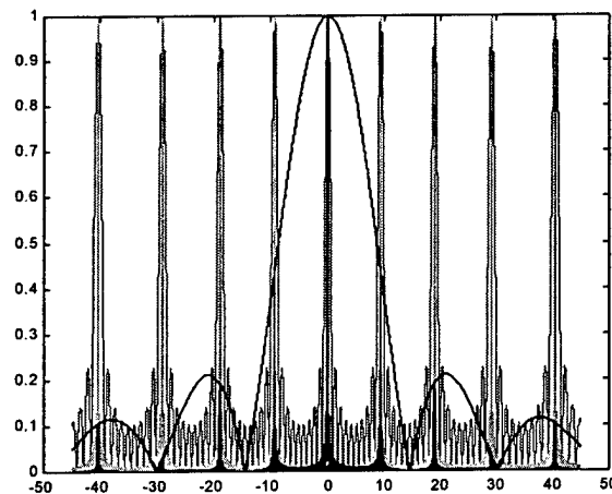
Figure 6.3-11. Comparison of Sidelobes for 100-Element and 10-Element Arrays, S_\lambda = 6.17\lambda . Purple (dark) line depicts 10-element PF; orange (light): 100-element PF. Single element pattern (black) and resultant 100-element SWA array pattern (blue) also shown.
