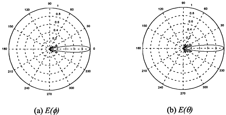
Figure 6.2-3. Polar Plots of E -fields for 64-Element Slotted Waveguide Array.
