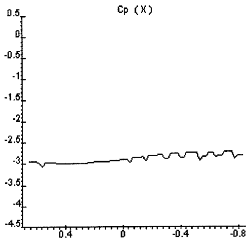
Corrected C_p distribution along wing span, section x=0.22 , M=0.3 , AOA=10^\circ
