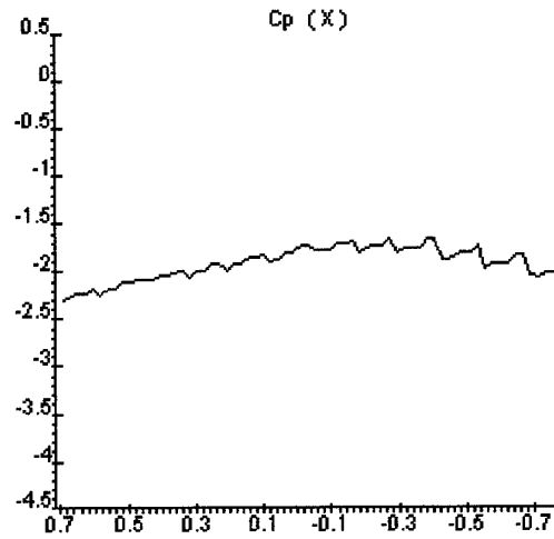
Non-corrected C_p distribution along wing span, section x=0.22 , M=0.3 , AOA=10^\circ
