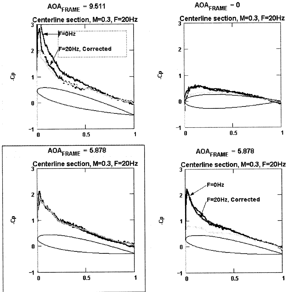
Fig.22. Comparison of the C_p distributions for F=0Hz and F=20Hz (corrected and source) M=0.3 .
