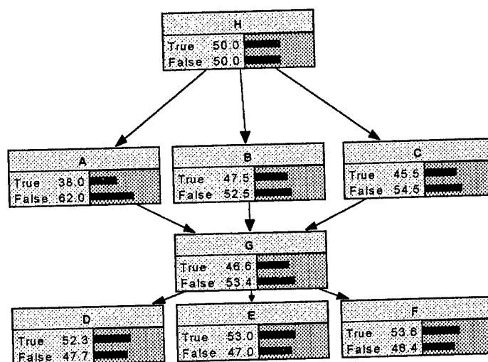
Figure 5-2 1X3X3 Network with Hidden Variable
