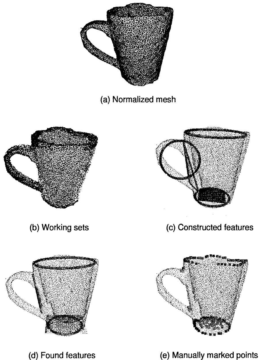
Figure 6.7: Processing stages for cup 2 with a mesh resolution (a) of 20K faces. The working sets are shown in (b) as red-convex, cyan-concave, green-planar, and yellow-other. In (c), circular constructed features are shown in red, planar constructed features are shown in blue, and line group constructed features are shown in orange. Found features are shown in (d). The rim is green, bottom edge is magenta, bottom surface plane is cyan, and the handle feature is orange. Part (e) shows the manually marked points used in quantitative testing.
