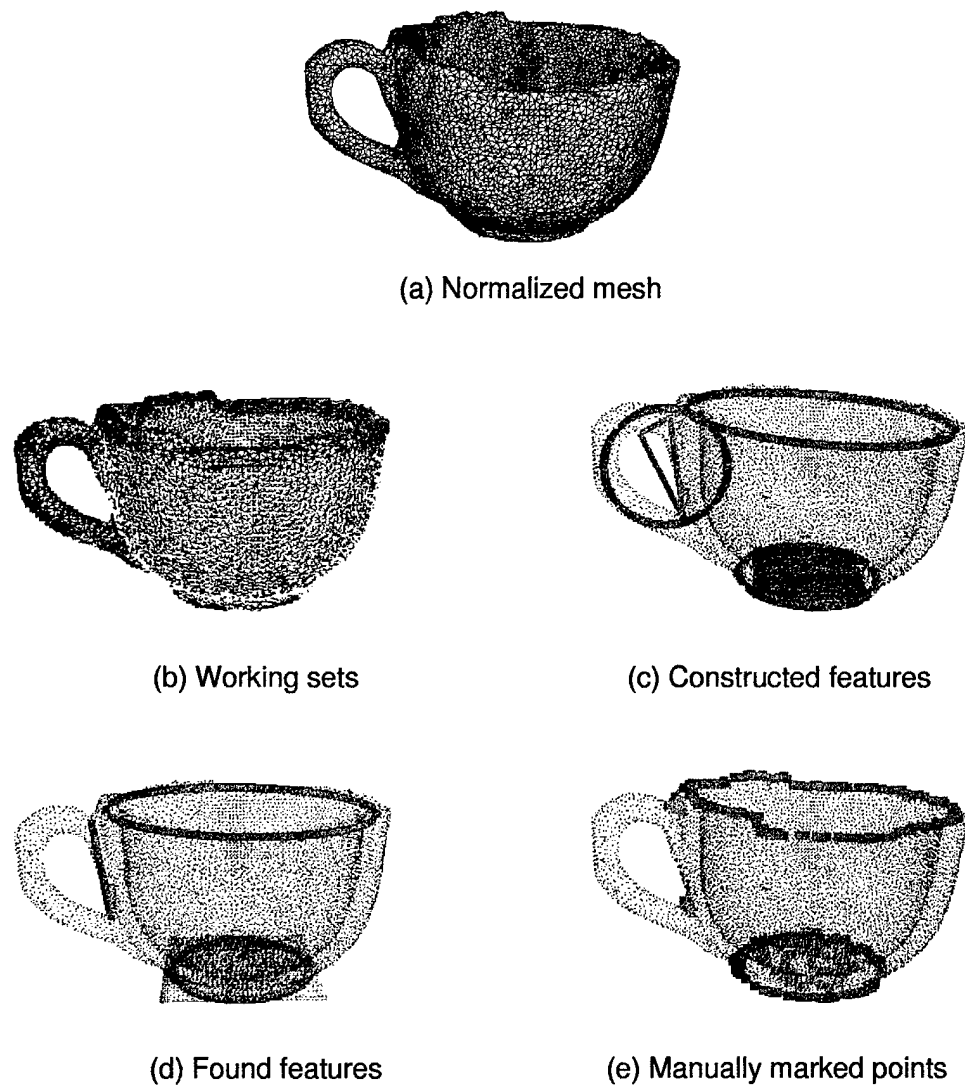
Figure 6.10: Processing stages for cup 3 with a mesh resolution (a) of 20K faces. The working sets are shown in (b) as red-convex, cyan-concave, green-planar, and yellow-other. In (c), circular constructed features are shown in red, planar constructed features are shown in blue, and line group constructed features in orange. Found features are shown in (d). The rim is green, bottom edge is magenta, bottom surface plane is cyan, and the handle feature is orange. Part (e) shows the manually marked points used in quantitative testing.
