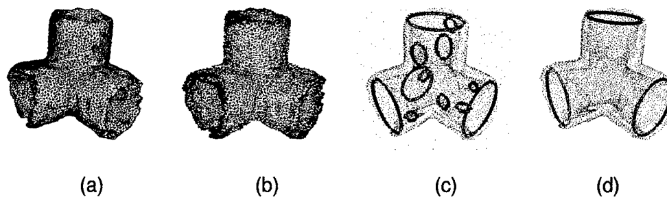
Figure 6.33: Processing stages for tricorner pipe fitting with a mesh resolution (a) of 20K faces. The working sets are shown in (b) as red-convex, cyan-concave, green-planar, and yellow-other. In (c), circular constructed features are generated using the convex working sets, and are shown in red. Found features are shown in (d).
