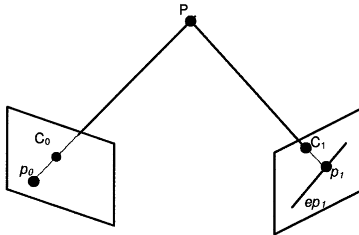
Figure 2.4: Epipolar geometry. p_0 is the image of point P . C_0, C_1 are the optical centers of cameras 0 and 1. The corresponding image point p_1 in camera 1 must lie on the line ep_1 , which is the image of a ray cast from p_0 through C_0 .
