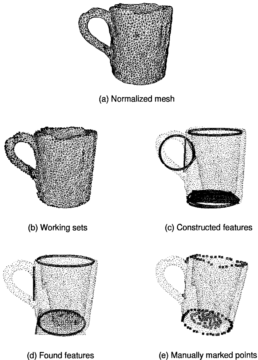
Figure 6.3: Processing stages for cup 1 with a mesh resolution (a) of 10K faces. The working sets are shown in (b) as red-convex, cyan-concave, green-planar, and yellow-other. In (c), circular constructed features are shown in red, planar constructed features are shown in blue, and line group constructed features in orange. Found features are shown in (d). The rim is green, bottom edge is magenta, bottom surface plane is cyan, and the handle feature is orange. Part (e) shows the manually marked points used in quantitative testing.
