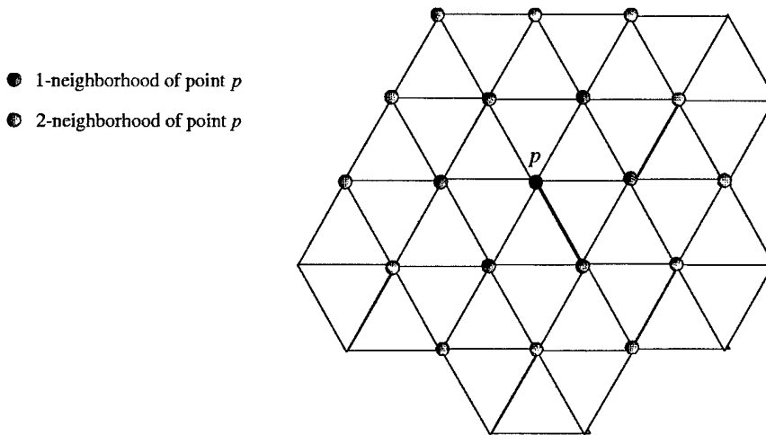
Figure 4.1: Neighborhoods defined on a partial mesh
