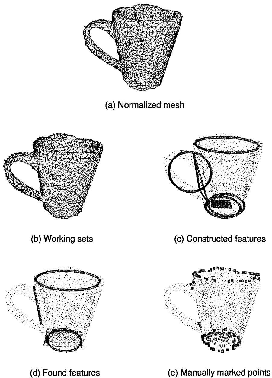
Figure 6.5: Processing stages for cup 2 with a mesh resolution (a) of 5K faces. The working sets are shown in (b) as red-convex, cyan-concave, green-planar, and yellow-other. In (c), circular constructed features are shown in red, planar constructed features are shown in blue, and line group constructed features in orange. Found features are shown in (d). The rim is green, bottom edge is magenta, bottom surface plane is cyan, and the handle feature is orange. Part (e) shows the manually marked points used in quantitative testing.
