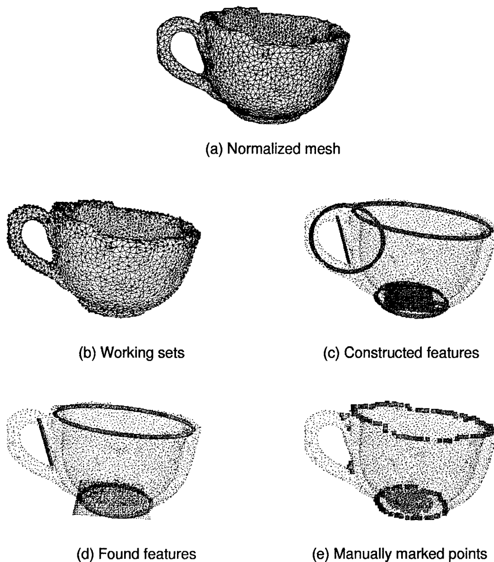
Figure 6.9: Processing stages for cup 3 with a mesh resolution (a) of 10K faces. The working sets are shown in (b) as red-convex, cyan-concave, green-planar, and yellow-other. In (c), circular constructed features are shown in red, planar constructed features are shown in blue, and line group constructed features in orange. Found features are shown in (d). The rim is green, bottom edge is magenta, bottom surface plane is cyan, and the handle feature is orange. Part (e) shows the manually marked points used in quantitative testing.
