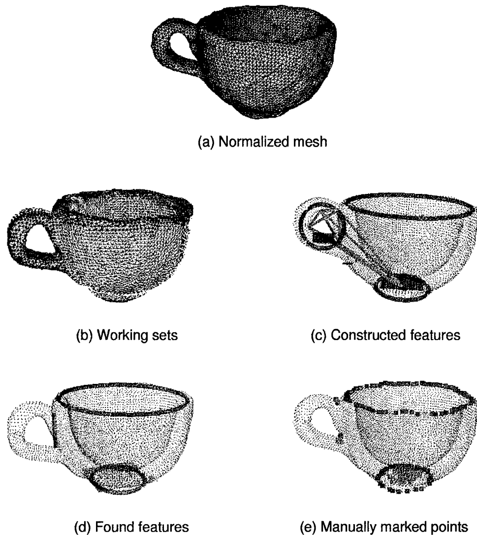
Figure 6.13: Processing stages for cup 4 with a mesh resolution (a) of 20K faces. The working sets are shown in (b) as red-convex, cyan-concave, green-planar, and yellow-other. In (c), circular constructed features are shown in red, planar constructed features are shown in blue, and line group constructed features in orange. Found features are shown in (d). The rim is green, bottom edge is magenta, bottom surface plane is cyan, and the handle feature is orange. Part (e) shows the manually marked points used in quantitative testing.
