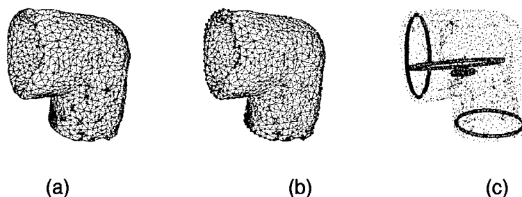
Figure 6.25: Processing stages for elbow pipe fitting with a mesh resolution (a) of 5K faces. The working sets are shown in (b) as red-convex, cyan-concave, green-planar, and yellow-other. In (c), circular constructed features are generated using the convex working sets, and are shown in red. In this case the object could not be identified, so no found features are displayed.
