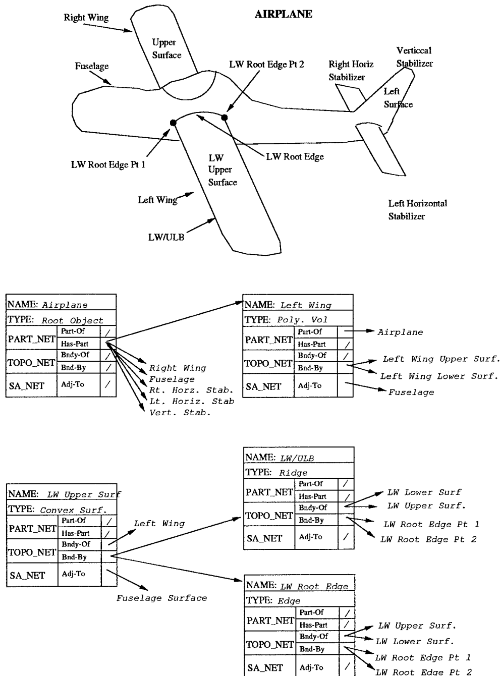
Figure 3.3: Abstract Model of Airplane. Due to complexity, only a partial model is shown here.
