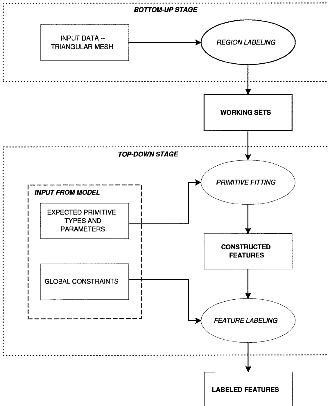
Figure 1.1: The proposed methodology for model-directed 3D feature extraction.
