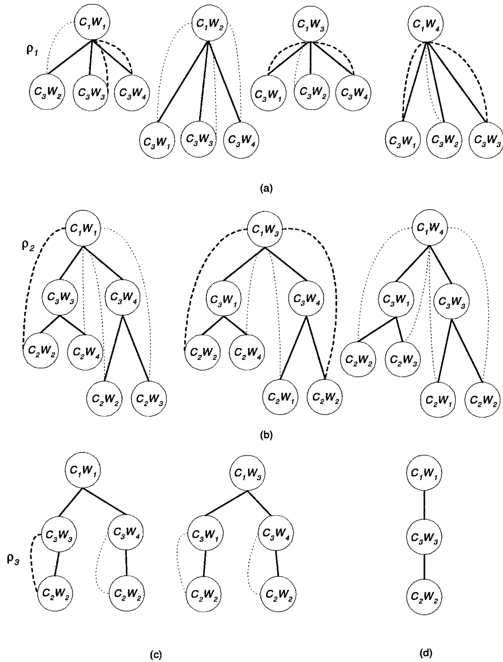
Figure 3.7: Example of constrained tree search using the working sets and features from Figure 3.6. Solid lines are potential labelings and dotted and dashed lines are constraint paths. Dashed lines indicate that a constraint is satisfied, while dotted lines indicate an unsatisfied constraint. (a) Before constraints are tested. (b) After \rho_1 tested. (c) After \rho_2 tested. (d) Final labeling after \rho_3 tested.
