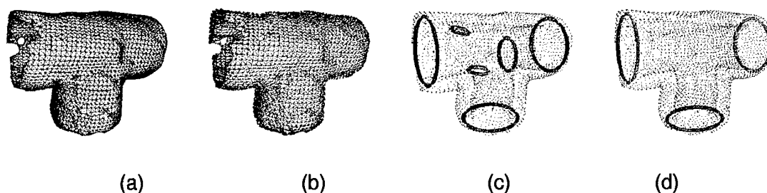
Figure 6.29: Processing stages for tee pipe fitting with a mesh resolution (a) of 10K faces. The working sets are shown in (b) as red-convex, cyan-concave, green-planar, and yellow-other. In (c), circular constructed features are generated using the convex working sets, and are shown in red. Found features are shown in (d) with both circles of a parallel pair shown in the same color and circles of a perpendicular pair shown in contrasting colors.
