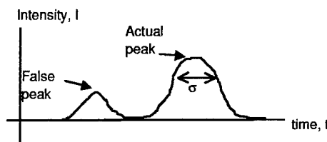
Figure 2.7: Peak intensity for a pixel. Time of actual peak intensity for each pixel is stored. False peaks are caused by inter-reflections, and must be removed.
