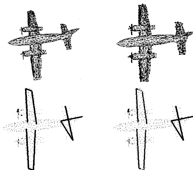
Figure 6.18: Processing stages for synthetic airplane. The working sets are shown as red-convex, cyan-concave, green-planar, and yellow-other. The line group constructed features are shown in blue. The labeled features are shown in orange. Only the wing edges were detected.
