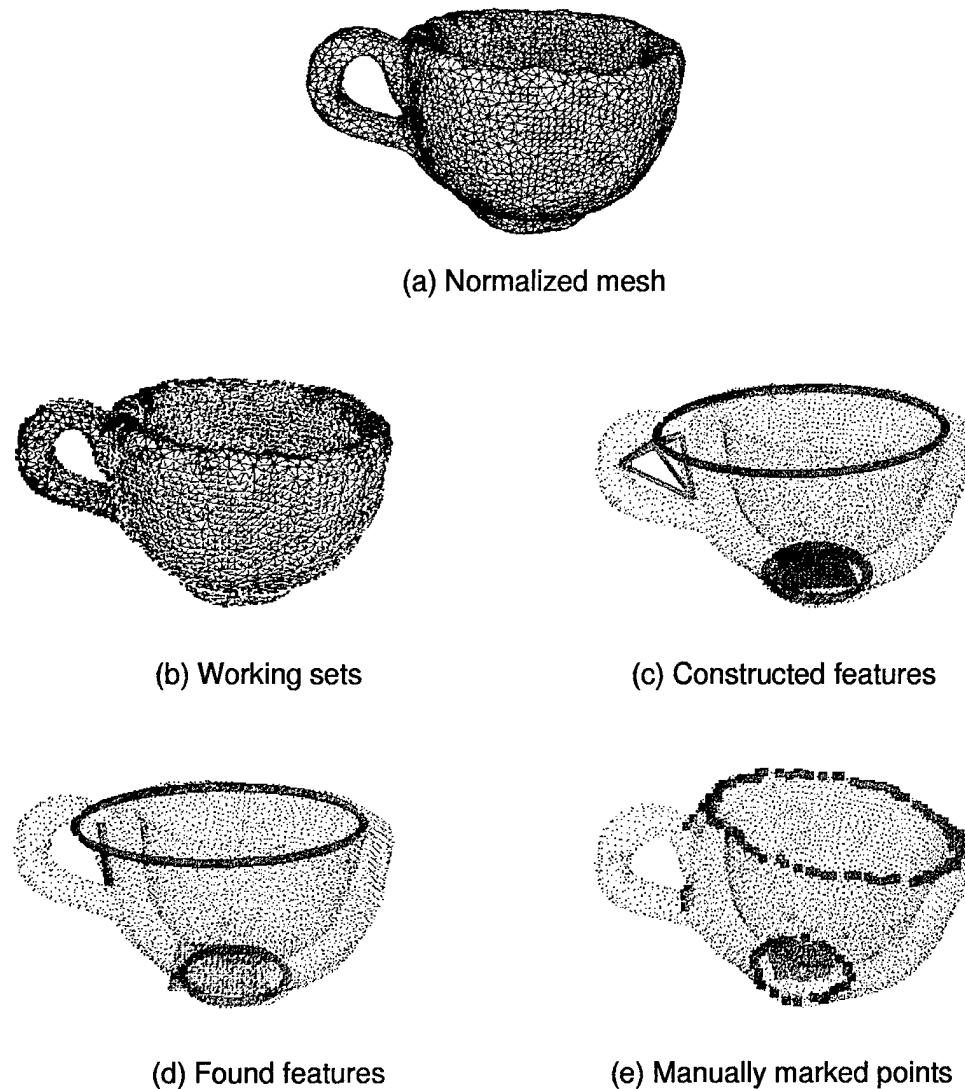
Figure 6.12: Processing stages for cup 4 with a mesh resolution (a) of 10K faces. The working sets are shown in (b) as red-convex, cyan-concave, green-planar, and yellow-other. In (c), circular constructed features are shown in red, planar constructed features are shown in blue, and line group constructed features in orange. Found features are shown in (d). The rim is green, bottom edge is magenta, bottom surface plane is cyan, and the handle feature is orange. Part (e) shows the manually marked points used in quantitative testing.
