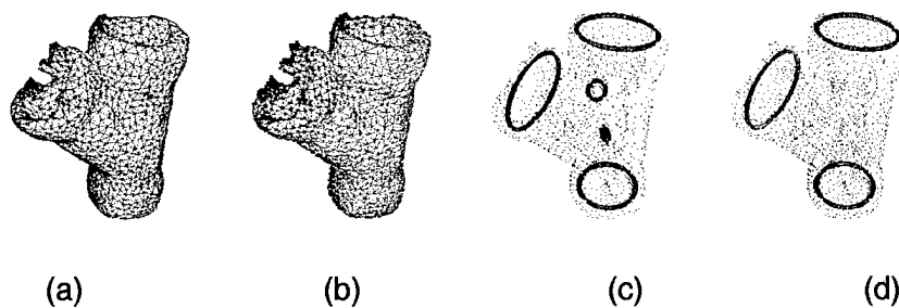
Figure 6.34: Processing stages for wye pipe fitting with a mesh resolution (a) of 5K faces. The working sets are shown in (b) as red-convex, cyan-concave, green-planar, and yellow-other. In (c), circular constructed features are generated using the convex working sets, and are shown in red. Found features are shown in (d).
