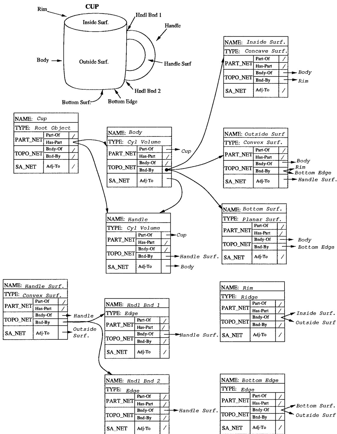
Figure 3.2: Abstract Model of Coffee Cup.
