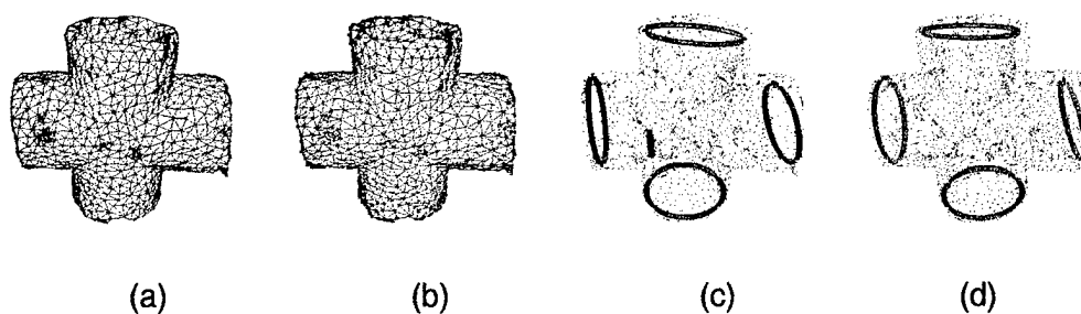
Figure 6.22: Processing stages for cross pipe fitting with a mesh resolution (a) of 5K faces. The working sets are shown in (b) as red-convex, cyan-concave, green-planar, and yellow-other. In (c), circular constructed features are generated using the convex working sets, and are shown in red. Found features are shown in (d) with both circles of a parallel pair shown in the same color and circles of a perpendicular pair shown in contrasting colors.
