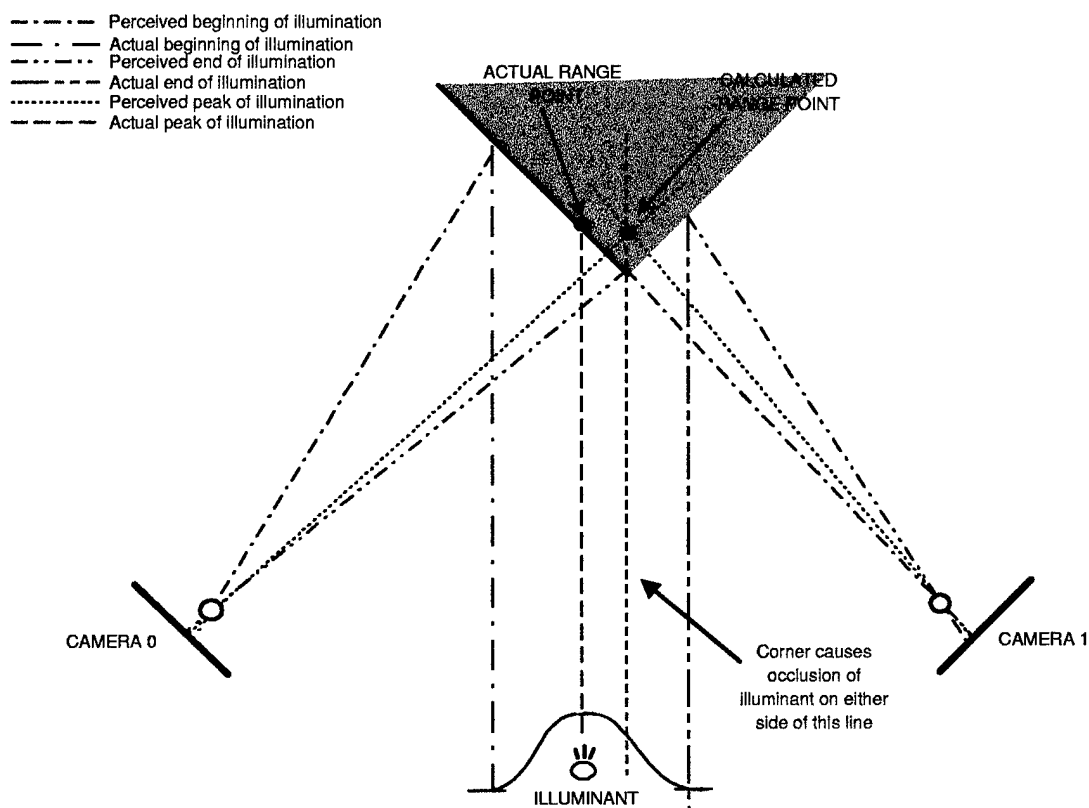
Figure 2.3: Range error in light striping system. Both cameras should map the center of the Gaussian intensity peak to the same pixel. The corner causes all illumination right of the dashed line to be occluded from camera 0, and all illumination left of the dashed line to be occluded from camera 1. This causes an erroneous depth calculation.
