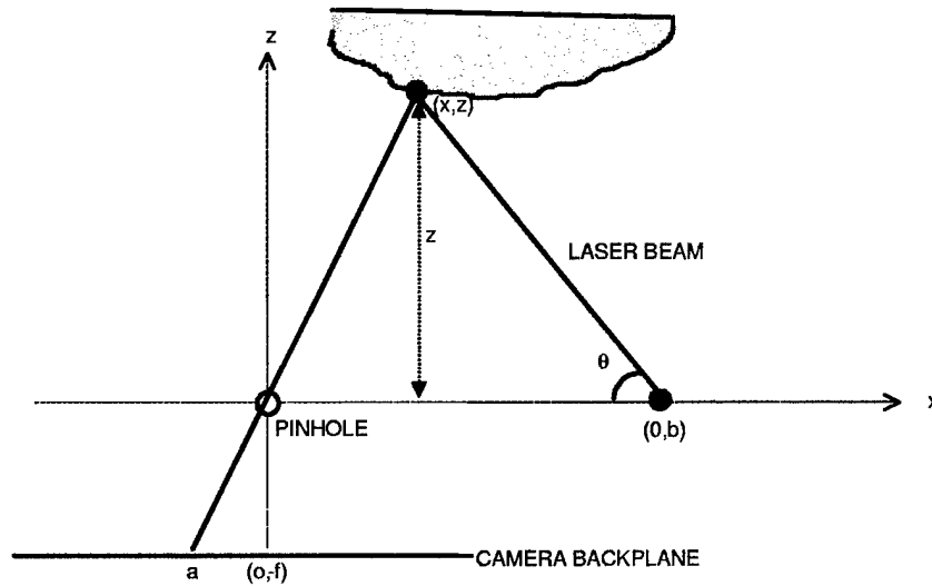
Figure 2.1: Optical triangulation geometry in 2-D. The camera, object and laser position are all fixed, and the positions are known. The laser angle, \theta , is varied to sweep the spot over the surface. The coordinates (x, z) can be calculated by simple trigonometry.
