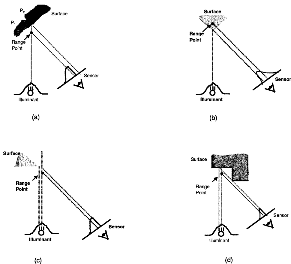
Figure 2.2: Range errors using traditional triangulation methods. (a) Reflectance discontinuity. (b) Corner. (c) Shape discontinuity with respect to the illumination. (d) Sensor occlusion.
