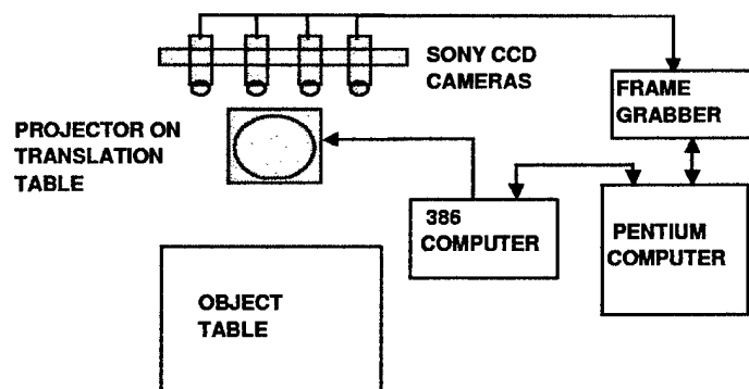
Figure 2.6: Physical setup of data acquisition system.
