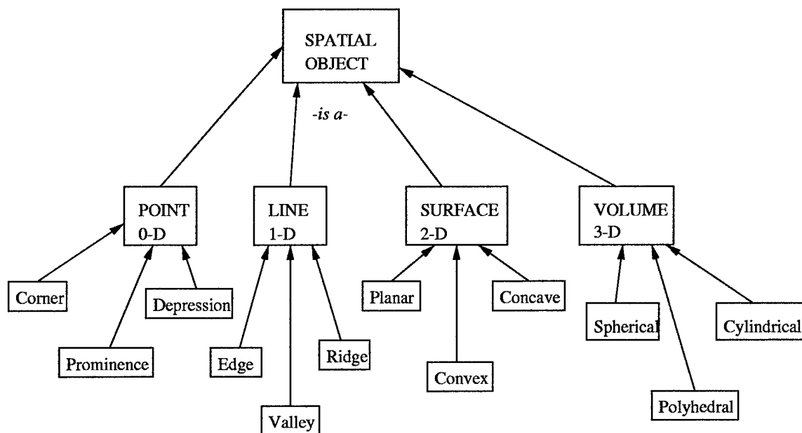
Figure 3.1: The Spatial Ontology.
