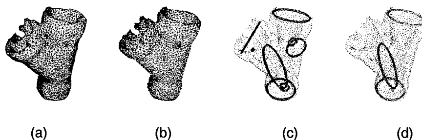
Figure 6.35: Processing stages for wye pipe fitting with a mesh resolution (a) of 10K faces. The working sets are shown in (b) as red-convex, cyan-concave, green-planar, and yellow-other. In (c), circular constructed features are generated using the convex working sets, and are shown in red. Found features are shown in (d).
