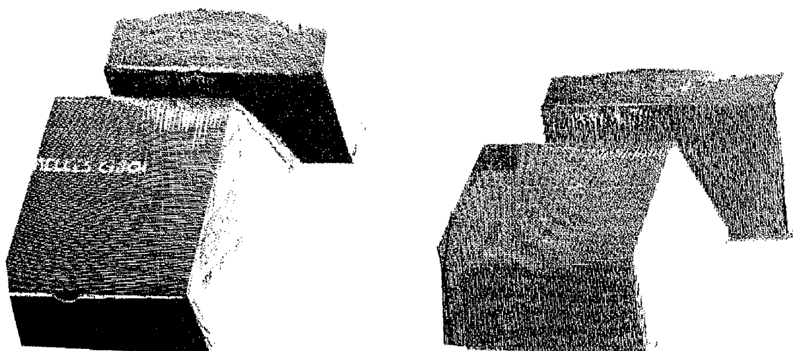
Figure 2.9: Boxes from figure 2.8 reconstructed using traditional (left) and spacetime (right) methods, with data obtained from cameras 0 and 3. Using traditional reconstruction, points on right side of near box must be erroneous since that face was occluded from camera 0. Also, note lack of data on top of box where words occur. On the spacetime reconstruction, observe that no points occur on the occluded face, and depth points are now present where words occur.
