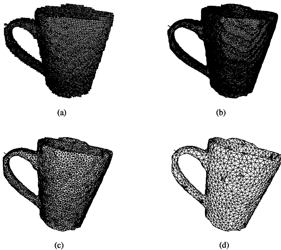
Figure 2.14: Mesh smoothing and normalization. (a) Initial mesh created by hierarchical space carving. (b) Results of smoothing operation. (c) Simplification to half the number of faces. (d) Simplification to 10% of the original number of faces.
