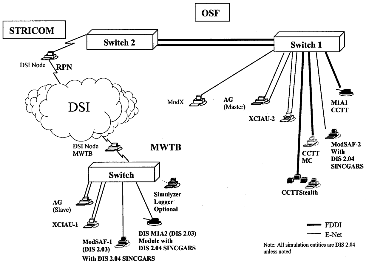
Figure 1 MWTB Test Configuration
