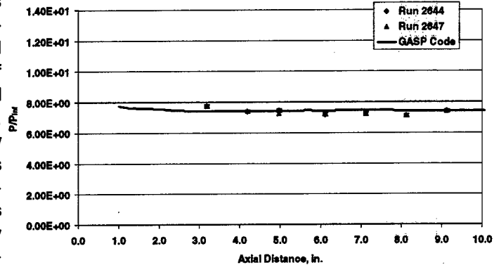
Fig. 12. Local environment pressure profile.
