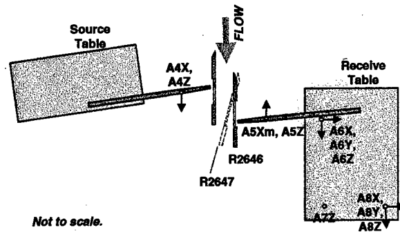
Fig. 16. T9 mechanical monitoring system setup.
