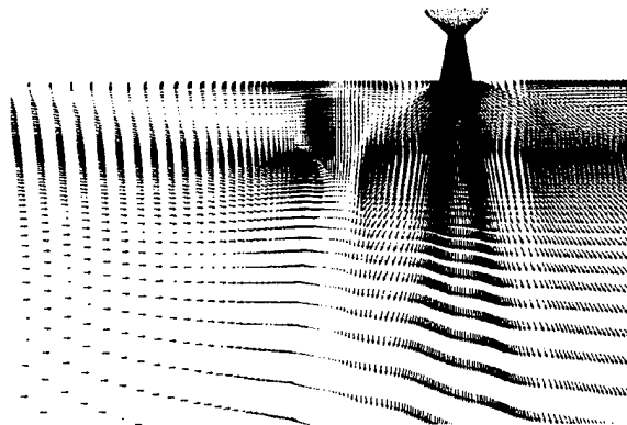
Fig. 17. Velocity vectors for 115-kft altitude, jet on case.
