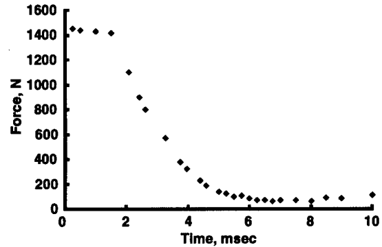
Fig. 22. Integrated normal force for jet turning off at 115-kft.
