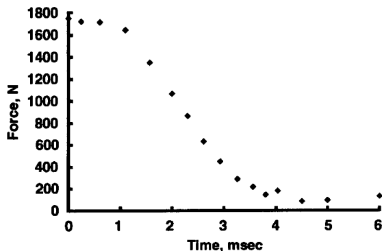
Fig. 13. Integrated normal force for jet turning off at 64.5 kft.
