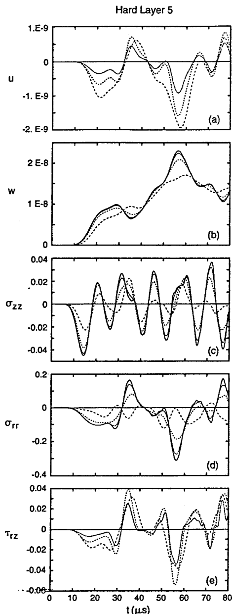
FIG. 11. Histories of hard layer 5 of basic stack: — r=0 , ---- r=r_p , ..... r=4r_p .
