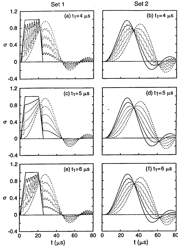
Fig. 8. Histories of \sigma in the first two sets of stack I with (h_A, h_B) = (0.49, 0.01) , t_f = 20 \mu s , \mathcal{J} = 1.034 : (a), (b) t_1 = 4 \mu s ; (c), (d) t_1 = 5 \mu s ; (e), (f) t_1 = 6 \mu s .
