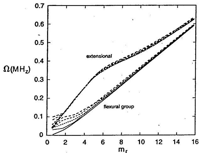
FIG. 3. Spectra of stack resonant frequency \Omega vs m , with massless bond (2-D model).
