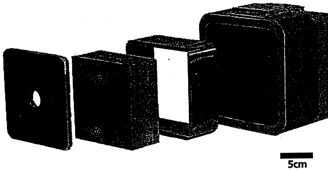
Fig. 3 Assembled AlN ceramic tiles and confinement components (test series 2)
