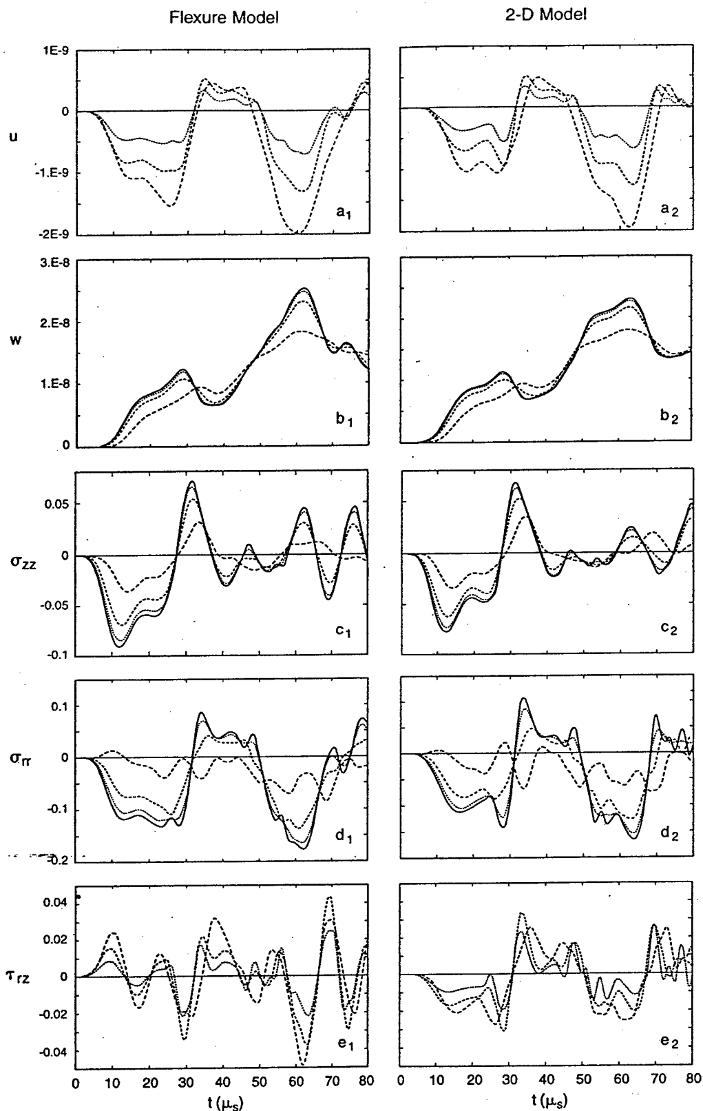
FIG. 6. Comparison of histories from the two models for disk 3: — r=0 ; ···· r=r_p ; ---- r=2r_p ; -.-.- r=4r_p .
