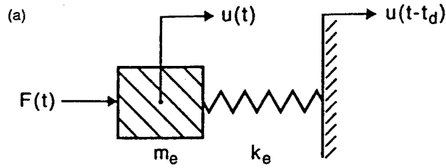
Fig. 10(a). Oscillator with moving base.
