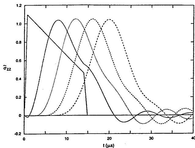
FIG. 5. Normalized \bar{\sigma}_{zz} histories from 1-D analysis with constant plan form area.
