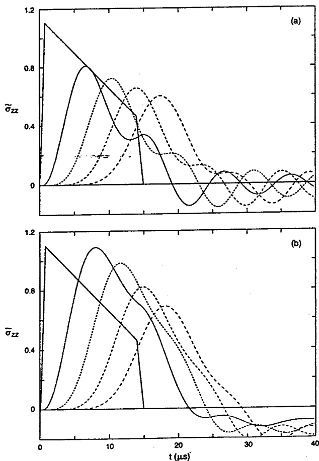
FIG. 6. Histories of \bar{\sigma}_{zz} in 1-D stack with 2 different plan form area distributions. (a) A_i/A_1 \rightarrow 1.0, 1.5, 1.9, 2.2, 2.5, 2.8, 3.1, 3.4, 3.7, 4.0 ; (b) A_i/A_1 \rightarrow 1.0, 1.0, 1.3, 1.8, 2.4, 3.0, 3.6, 4.0, 4.0, 4.0 .
