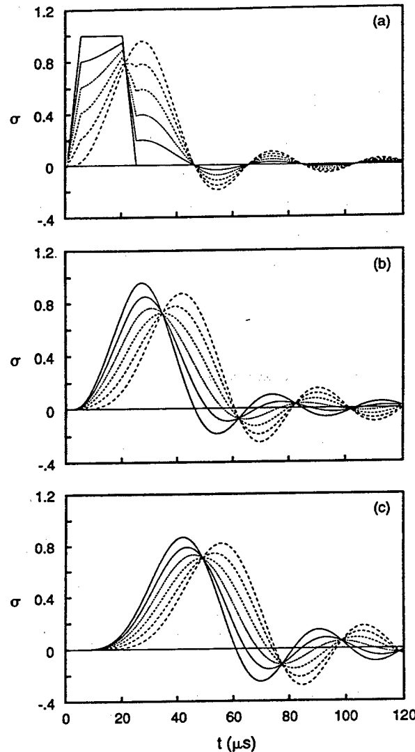
Fig. 2. Histories of \sigma within each of the first 3 sets of the basic stack with m_s = 20 , \mathcal{J} = 1.034 , t_f = 20 \mu s .
