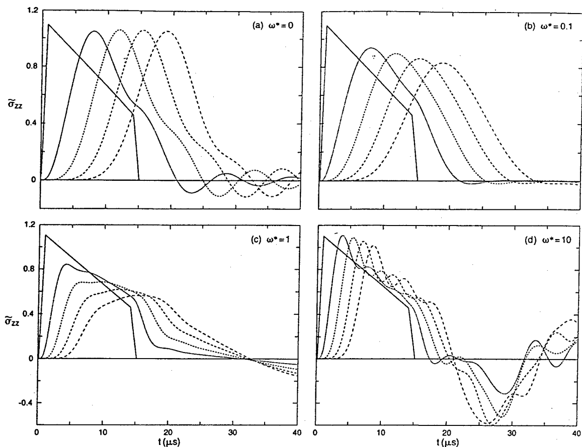
FIG. 10. Histories of \tilde{\sigma}_{zz} in 1-D stack with constant plan from area bonded by viscoelastic layers ( \omega^* = \omega_{set}\sqrt{\tau_\sigma\tau_\epsilon} ).
