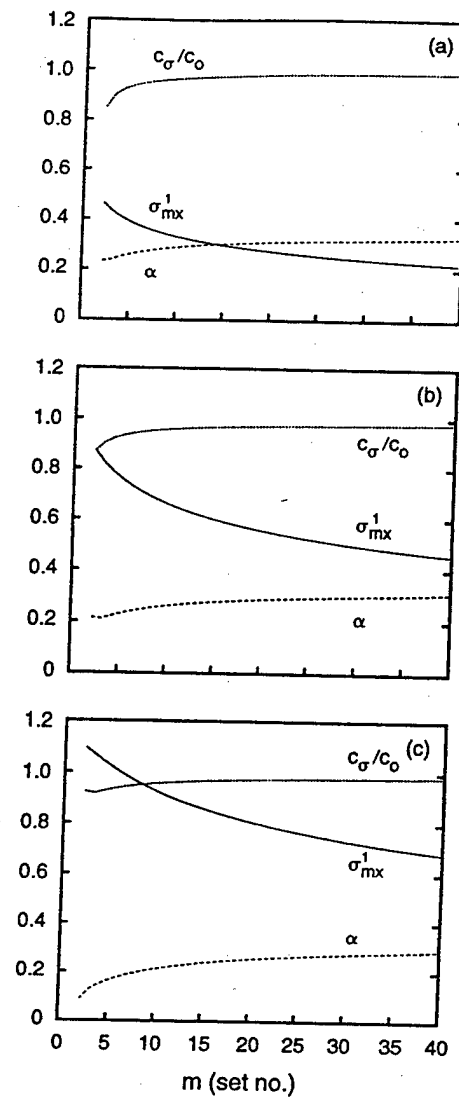
Fig. 7. Variation of \sigma_{mx}^1 , c_\sigma/c_0 and \alpha along stack with m_s = 48 , (a) J = 0.484 , (b) J = 1.040 , (c) J = 1.631 .
