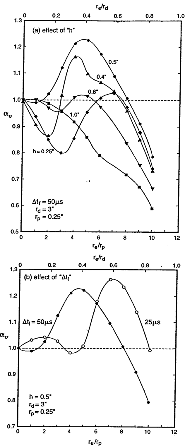
Figure 11: Variation of " \alpha_\sigma " with " r_e " for "simply supported edge"; r_d = 3"
