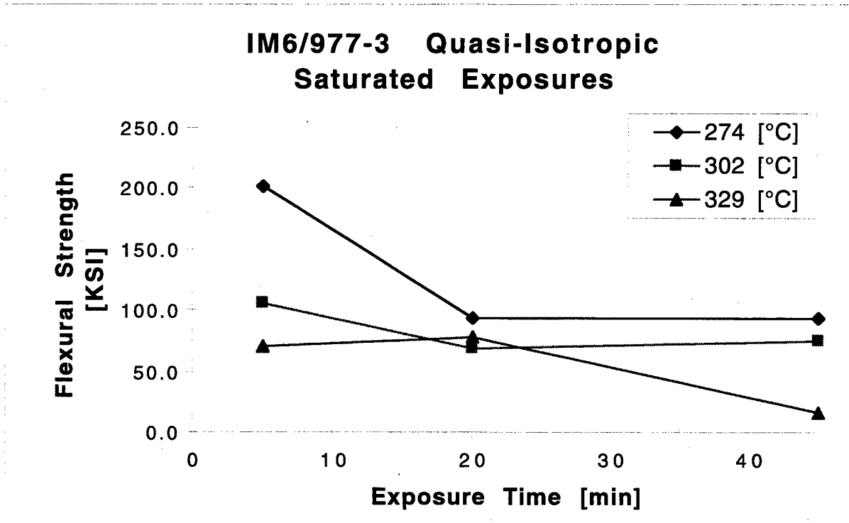
Figure B-48 FLEXURE RESULTS FOR SATURATED IM6/977-3 QUASI-ISOTROPIC COUPONS
