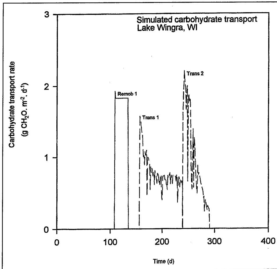
Figure 6. Simulated behavior of carbohydrate flow through plant compartments (Carbohydrate remobilization and upward transport from rhizomes/root crowns are used for initial growth of each plant cohort. Down-Ward carbohydrate translocation into rhizomes/root crowns occurs during anthesis and senescence of each plant cohort (Initial biomass and climatological data as in nominal run))
