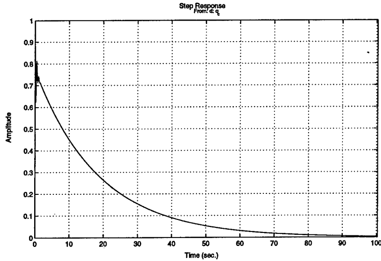
Figure 6.6: Pitch Rate Error Step Response: Based on Controller K_{qA}
