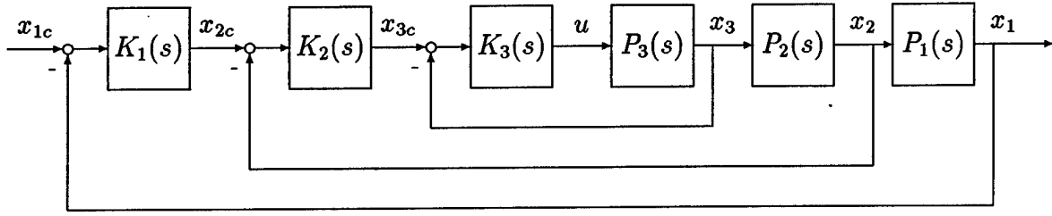
Figure 3.3: Decoupled System Architecture
