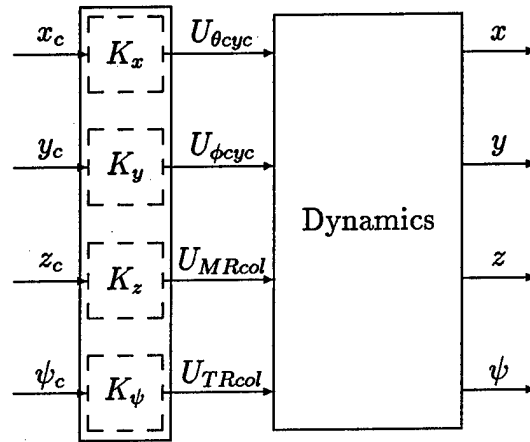
Figure 6.1: Entire DSAAV System of Coupled Channels
