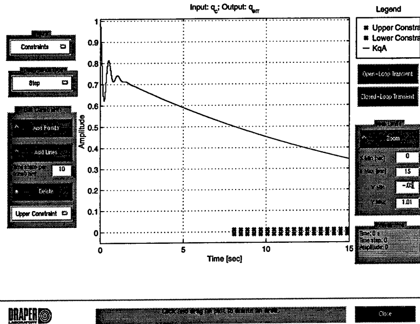
Figure 6.12: q_{err}(t) Step Response Constraint
