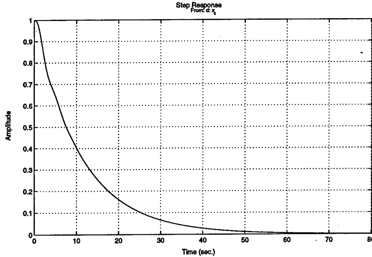
Figure 6.9: Forward Position Error Step Response: Based on Controller K_{xA}
