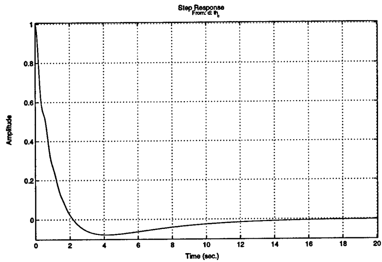
Figure 6.7: Pitch Error Step Response: Based on Controller K_{\theta A}
