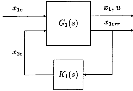
Figure 3.9: Outer Loop: Model Based Representation
