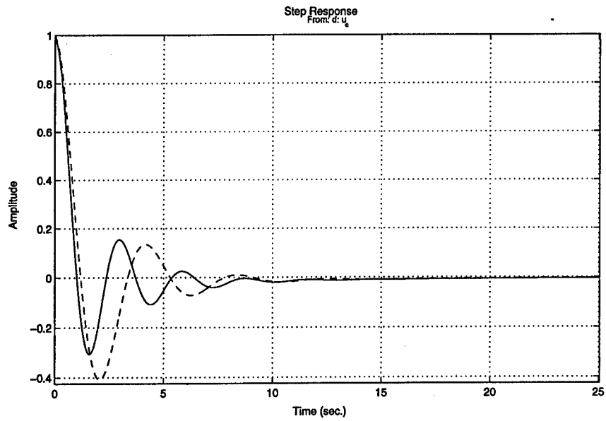
Figure 6.17: u_{err}(t) for Forward Velocity Controller Designs
