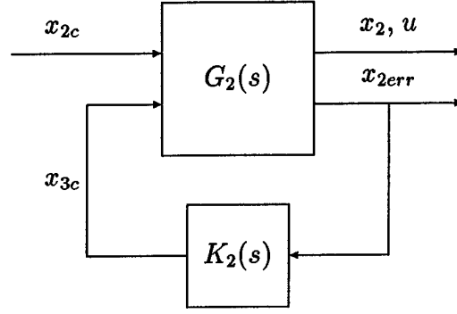
Figure 3.7: Intermediate Loop: Model Based Representation
