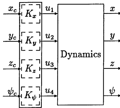
Figure 3.1: Entire System of Coupled Channels
