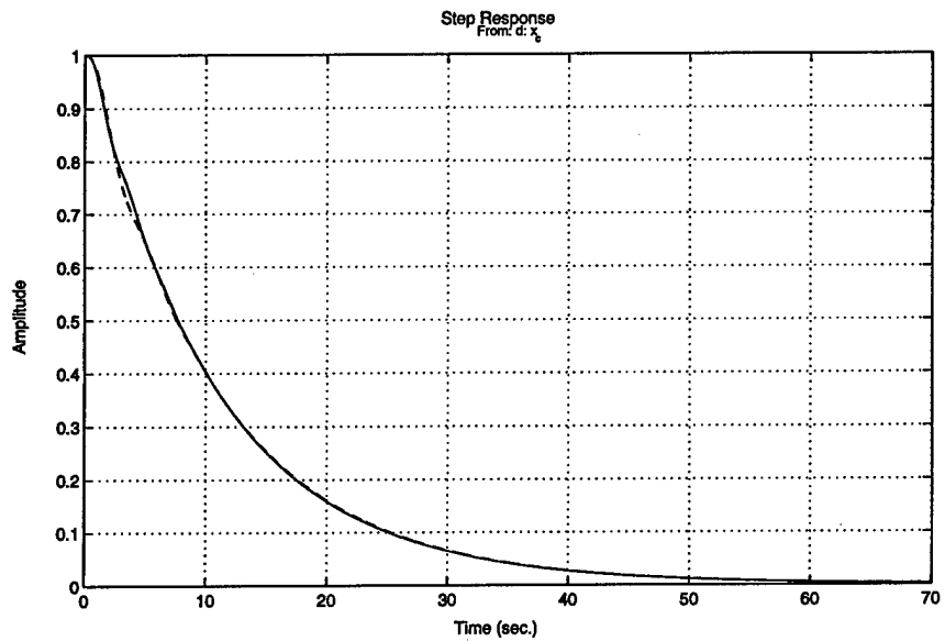
Figure 6.18: x_{err}(t) for Forward Position Controller Designs
