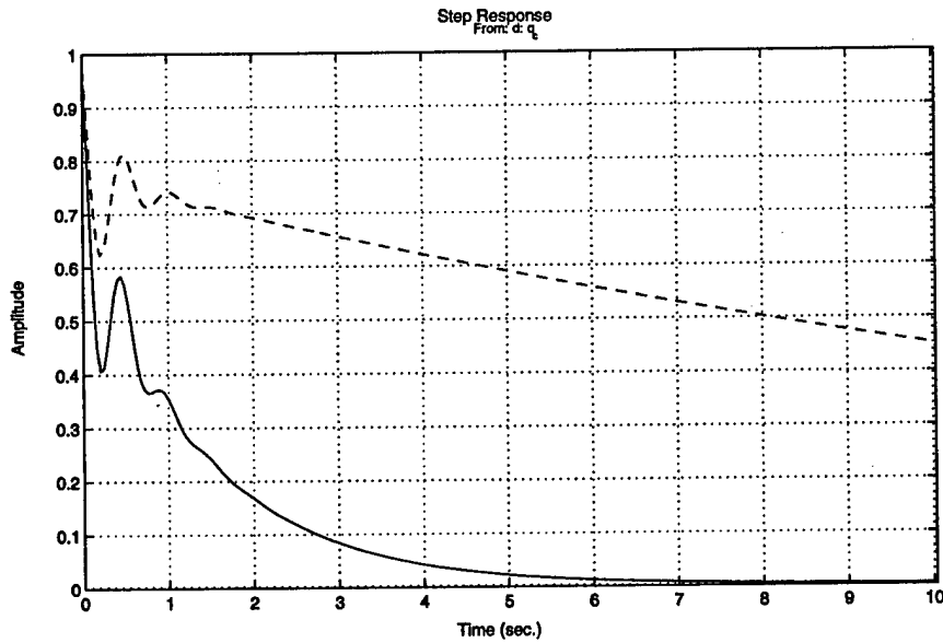
Figure 6.15: Step Responses for Pitch Rate Controller Designs
