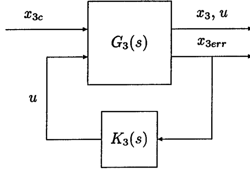
Figure 3.5: Innermost Loop: Model Based Representation
