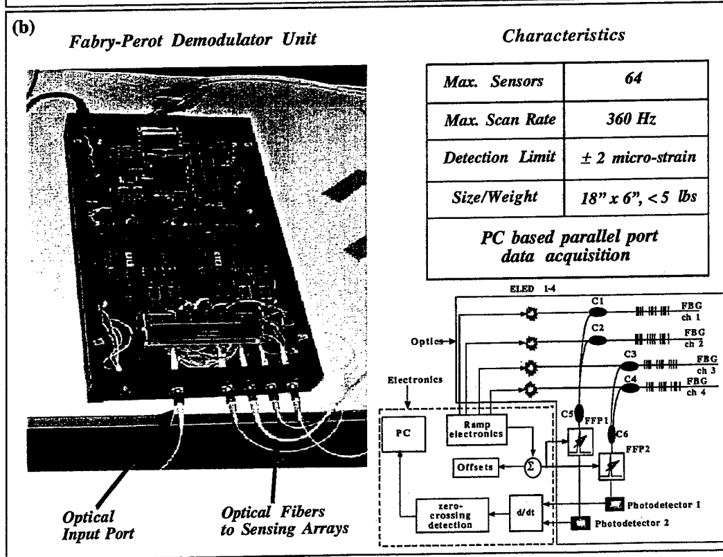
Figure 2. (a) Wavelength division multiplexing (WDM) strategy; (b) NRL Fabry-Perot WDM system, including schematic and performance characteristics.
