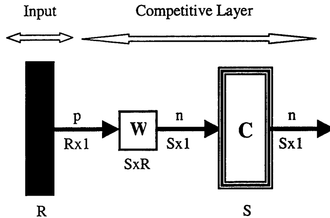
Figure 3.2 Competitive Neural Network
