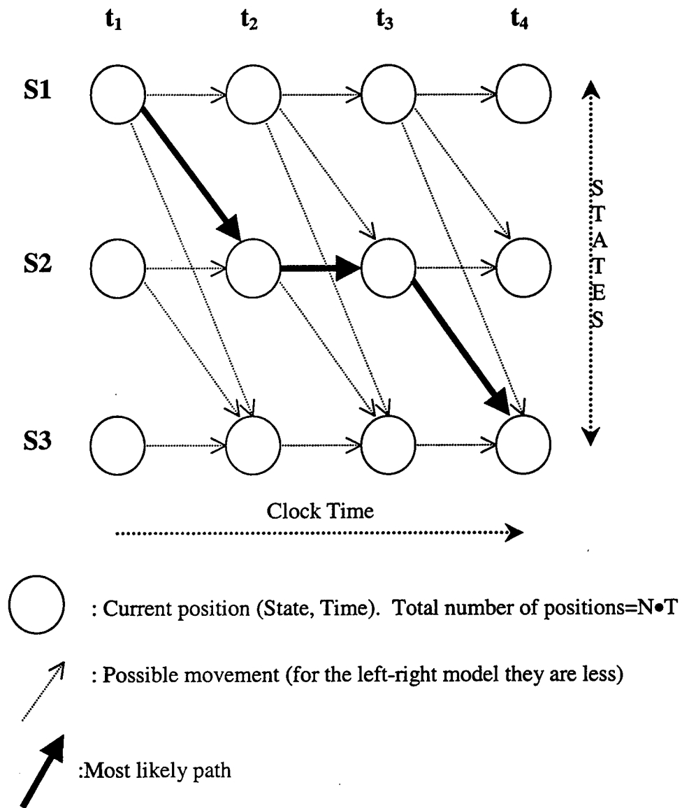
Figure 2.4b Trellis Diagram for T=4 , and N=3 , left-to-right model as used for example in Figure 2.3. Fewer possible paths than in ergotic model are allowed.
