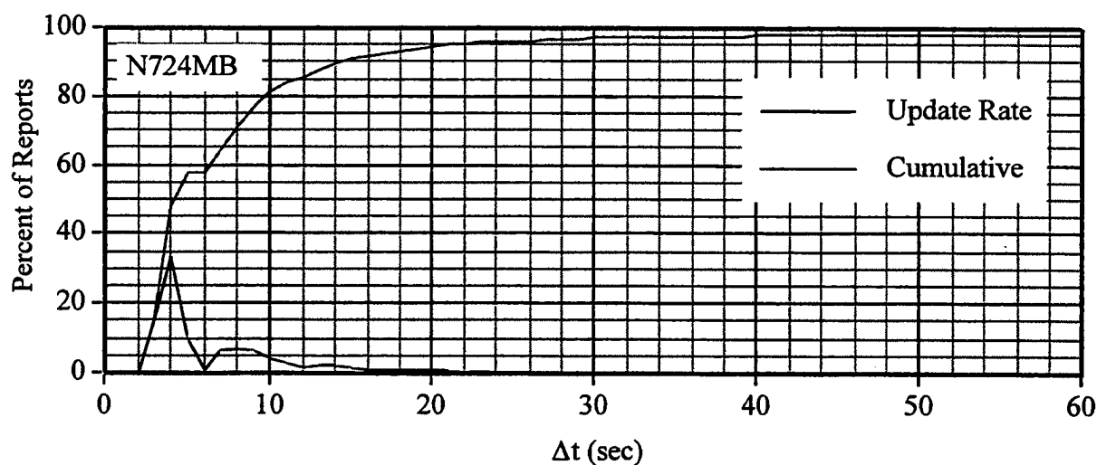
Figure 4.1 Position Report Update Rate
