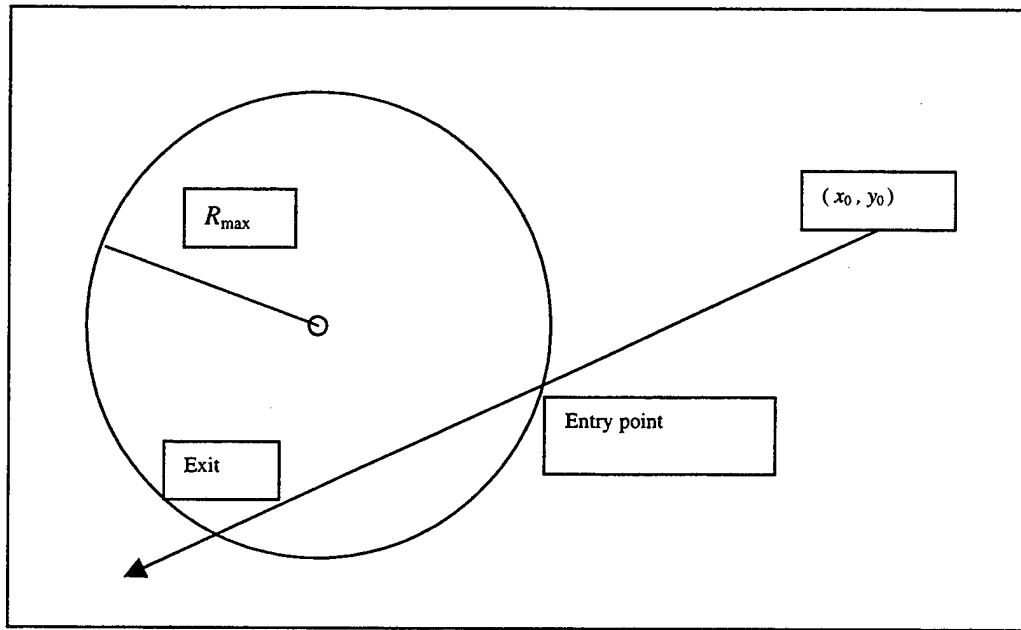
Figure 4.1. The Mover-Sensor Geometry
