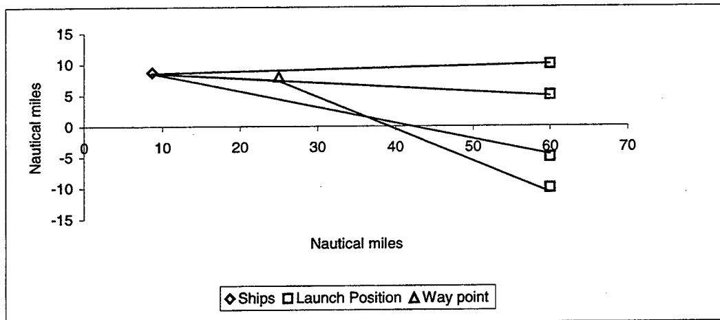
Figure 5.4. Launch Geometry with Minimum Spread and Long Range
