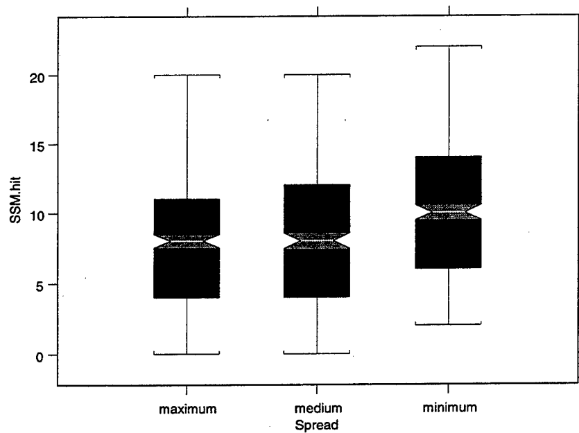
Figure 6.4. Boxplot of SSM Hits over Spread
