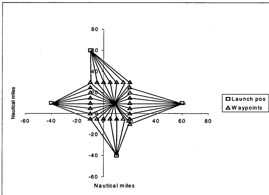
Figure 5.3. Launch Geometry with Maximum Spread and Long Range. The Target-ships are in the Center
