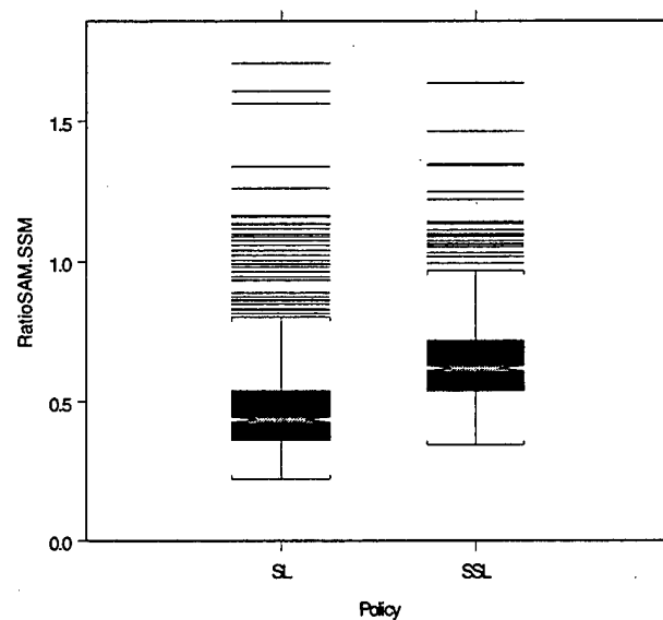
Figure 6.7. Boxplot of Success Ratio for SAM over Firing Policy
