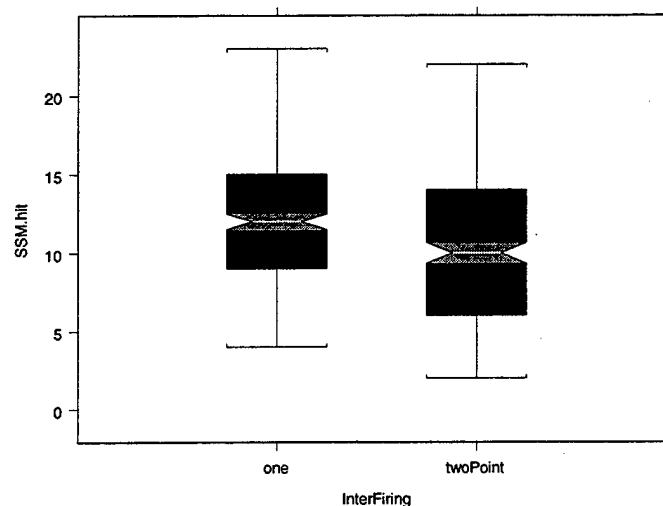
Figure 6.9. Boxplot for SSM Hits over Interfiring Delays 1 and 2.5 Seconds
