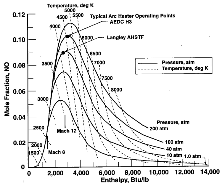
Fig. 2. Nitric oxide in high-temperature equilibrium air (NO) mole fraction vs. enthalpy at constant pressure. At all simulation Mach numbers lower than 12, cold air dilution will be required to match the enthalpy.
