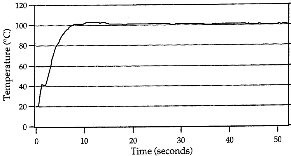
Figure 8. Induction System Response With PID Feedback Control.
