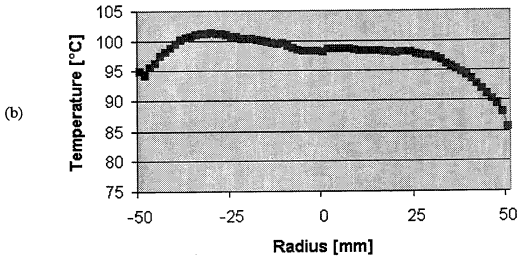
Figure 17. Surface Temperature Variation During Bonding of Ceramic Tile to 7/16-in-Thick Glass/Epoxy Composite With Coil Motion.
