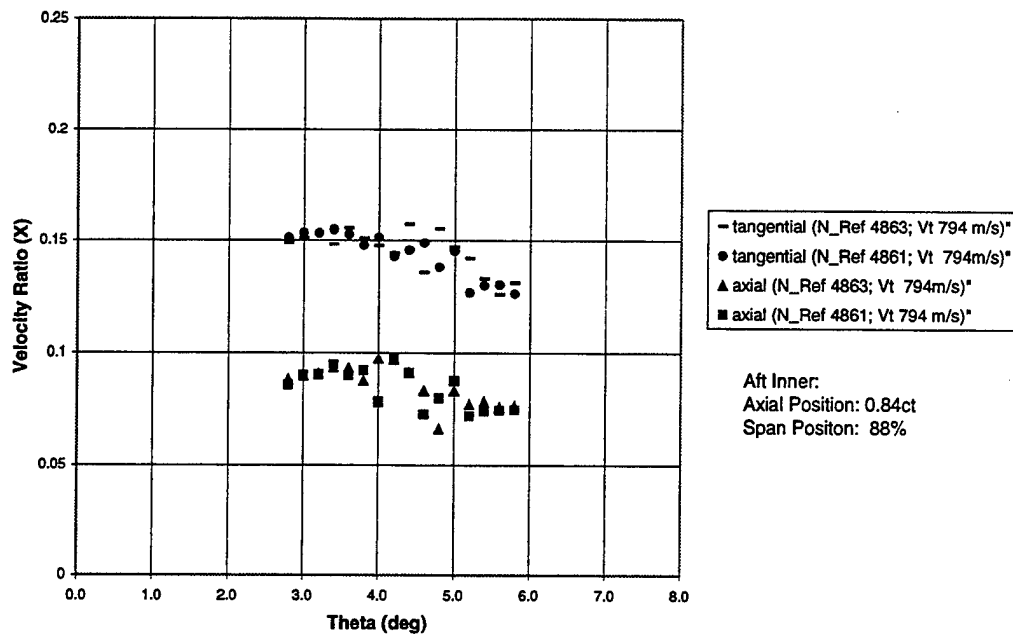
Figure 58. LDV Velocity Ratios for 0.84 c_t and 88% Span
